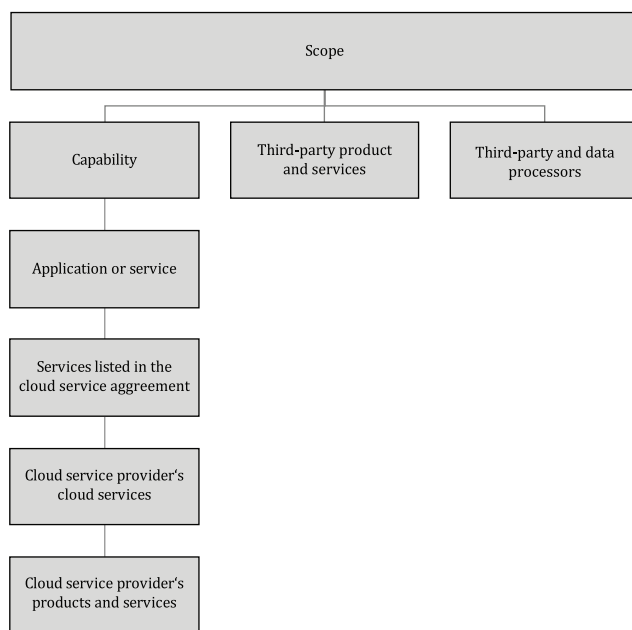
Figure 3 — Data usage scopes according to ISO/IEC 19944:2017
