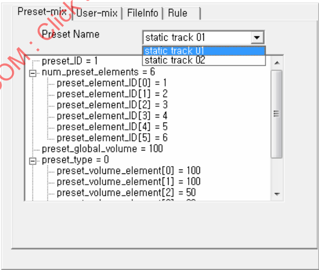
Figure D.3 — User interface of the browser for preset-mix mode (“Preset-mix”)
