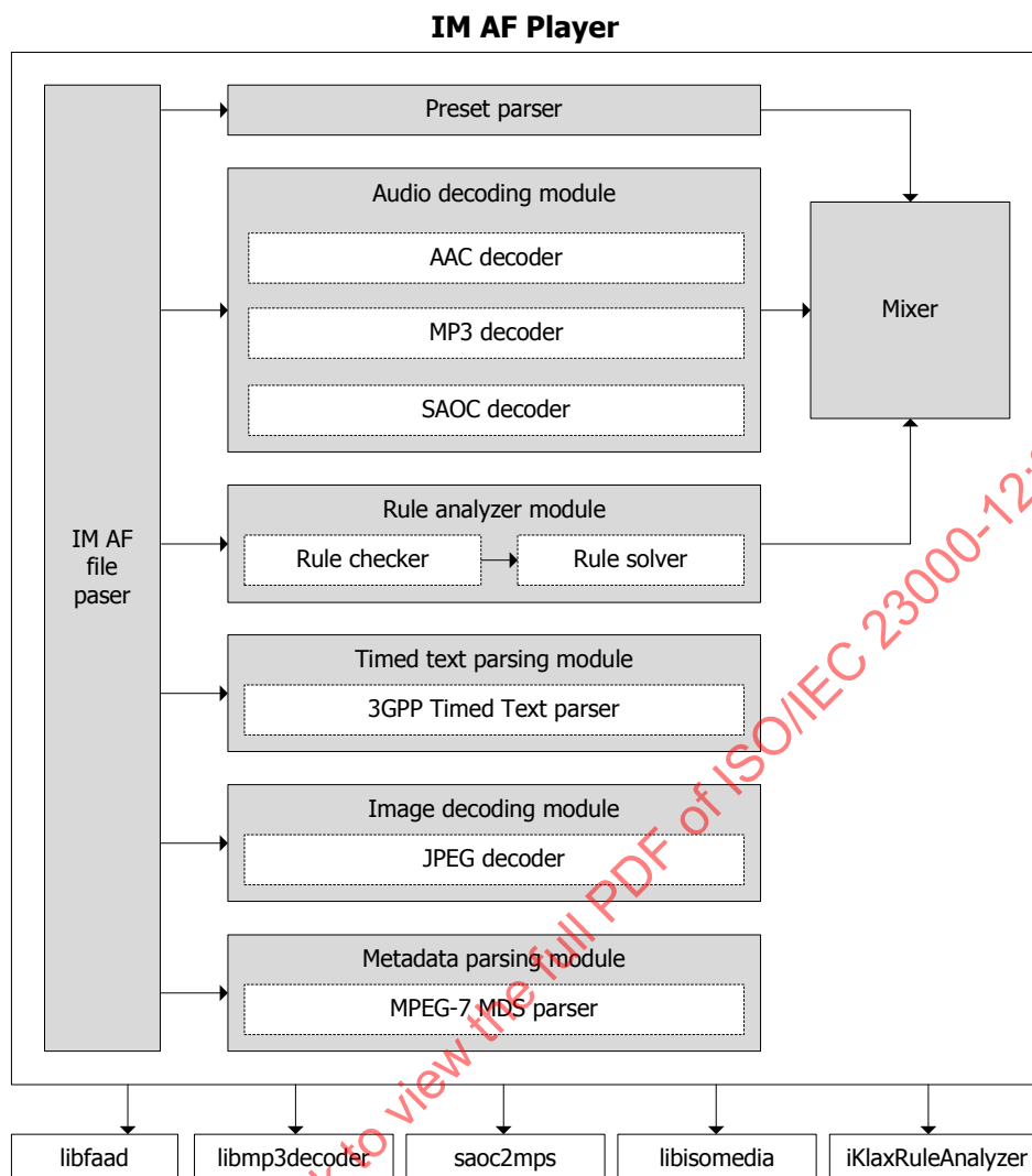
Figure AMD1.1 — The architecture of an Interactive Music AF player
