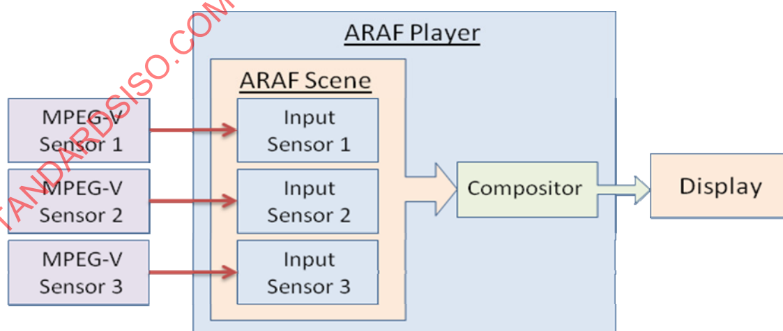
Figure 3 — Diagram of the architecture for accessing MPEG-V sensor data
