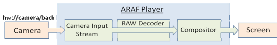
Figure 5 - Diagram of the architecture for accessing the camera frames
