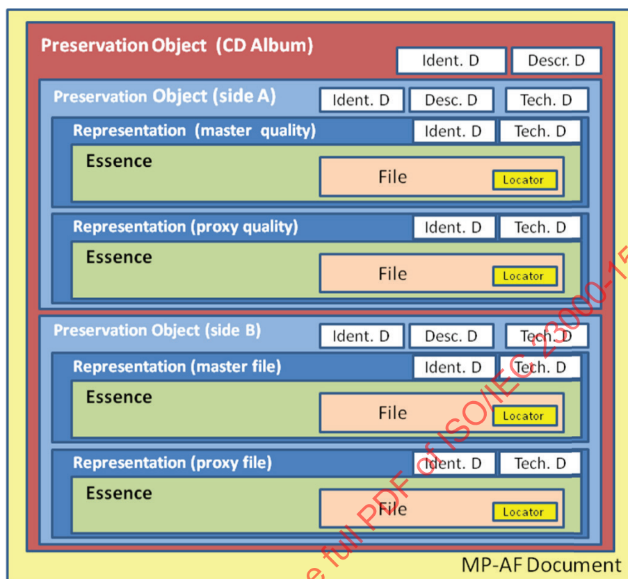
Figure 24 — Logical structure of the MP-AF Document as used by NDL
