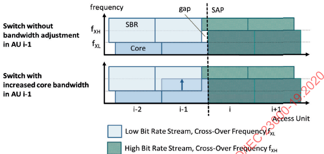
Figure 16 — Illustration of core bandwidth adjustment for HE-AAC switching points
