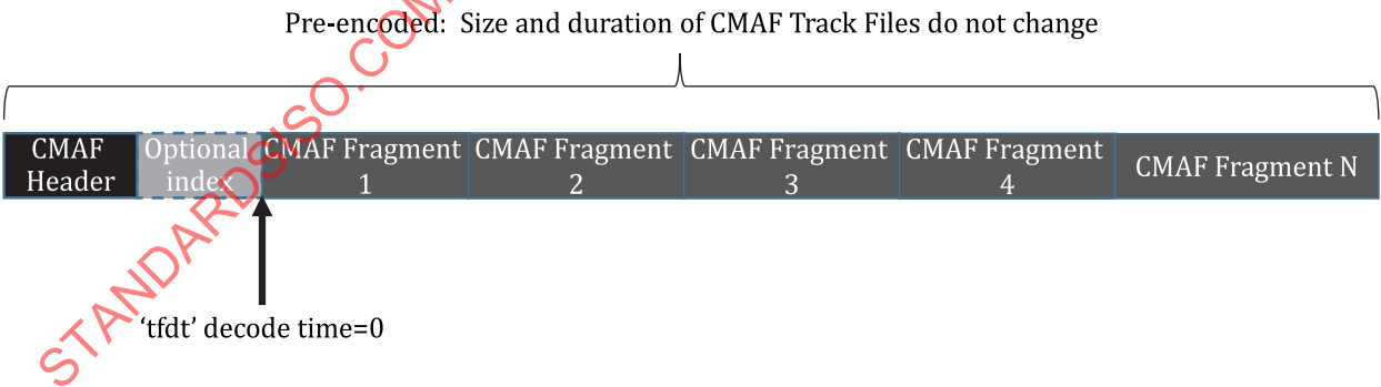
Figure 6 — CMAF track file, addressable media object
