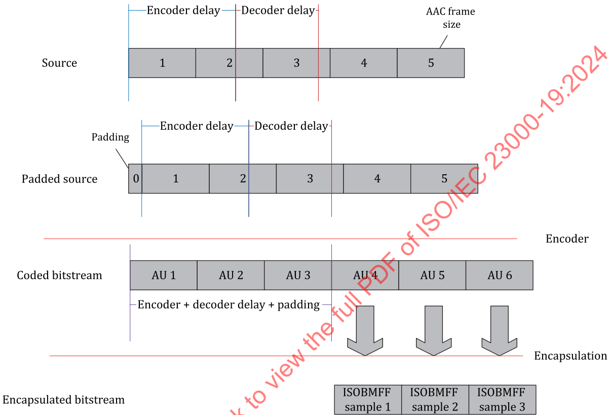
Figure G.1 — Example of padding and trimming AAC access units for delay compensation
