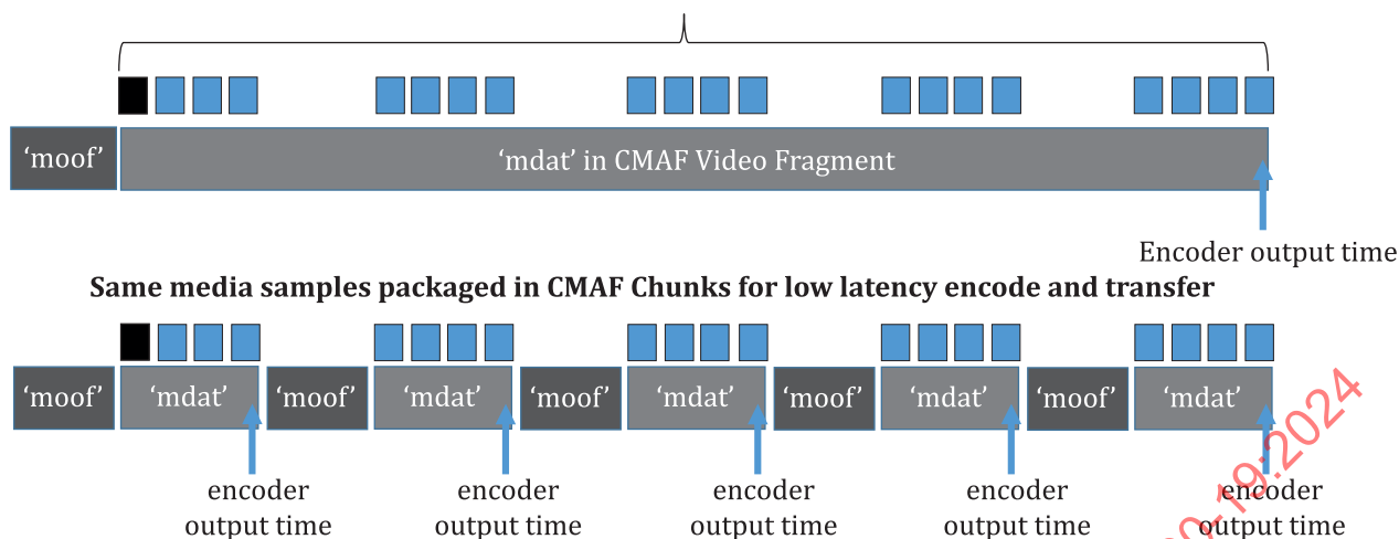
Figure 8 — CMAF chunk, addressable media objects
