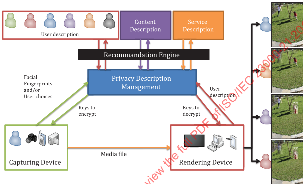
Figure 2 — Proposed framework for privacy management of media
