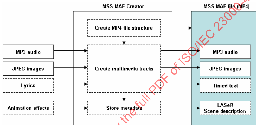
Figure 5 — Example of Musical slide show application format creator system architecture
