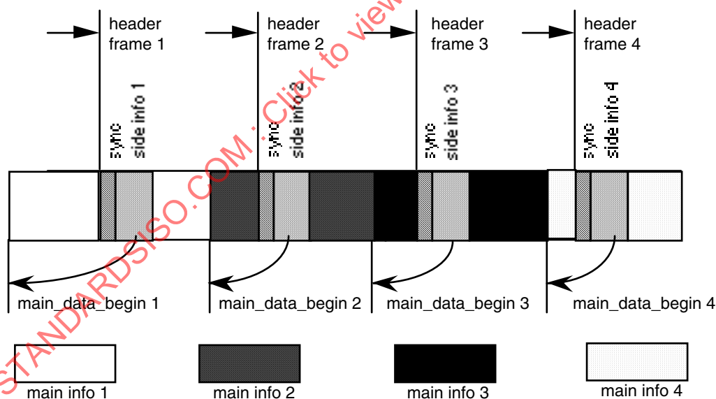
Figure 1 — Layer 3 bit stream organization
