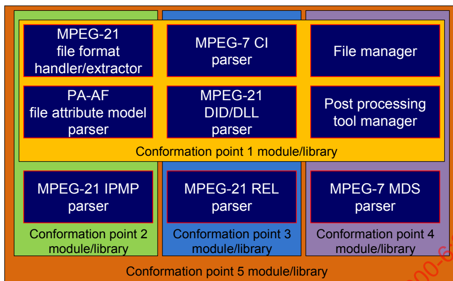
Figure AMD1.4 — A PA-AF file extractor software modules
