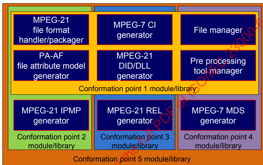
Figure AMD1.2 — PA-AF packager/authoring tool software modules
