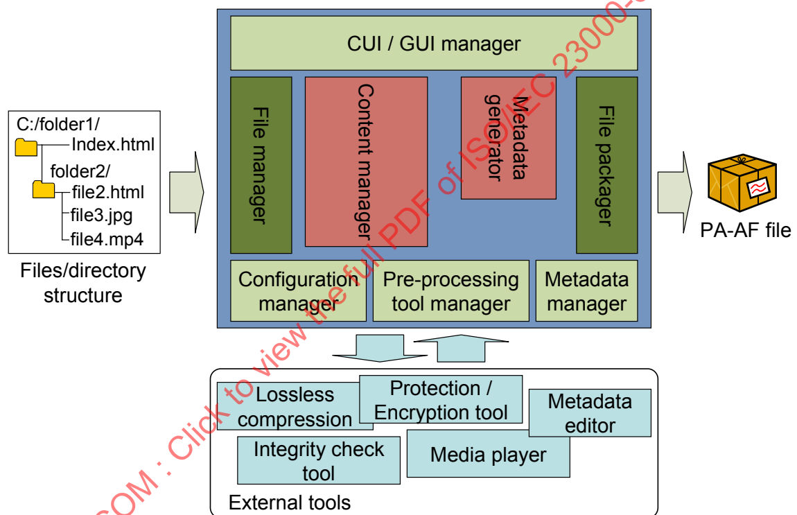
Figure AMD1.1 — A PA-AF packager/authoring tool architecture
