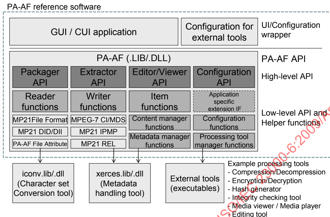
Figure H.1 — Overview of a sample PA-AF API structure
