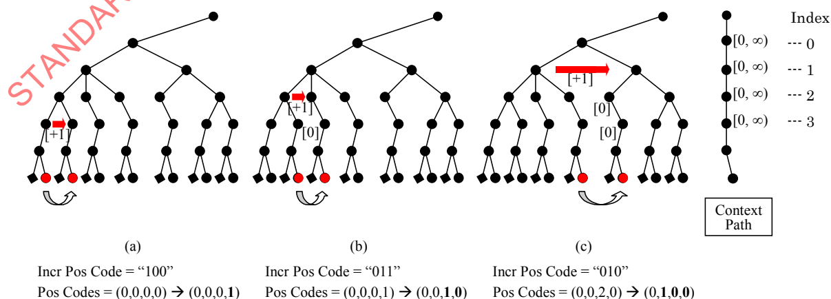
Figure 19 — Indicated Positions using Incremental Position Codes
