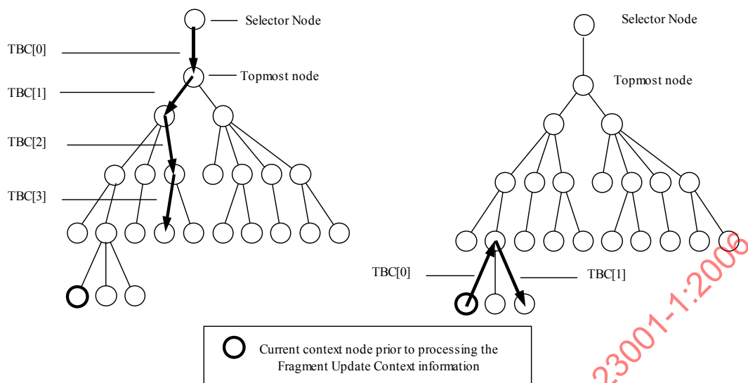
Figure 8 — Absolute (left) and relative context path example
