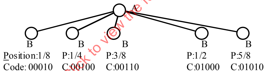
Figure 13 — Assignment of Position Codes to a set of child elements
