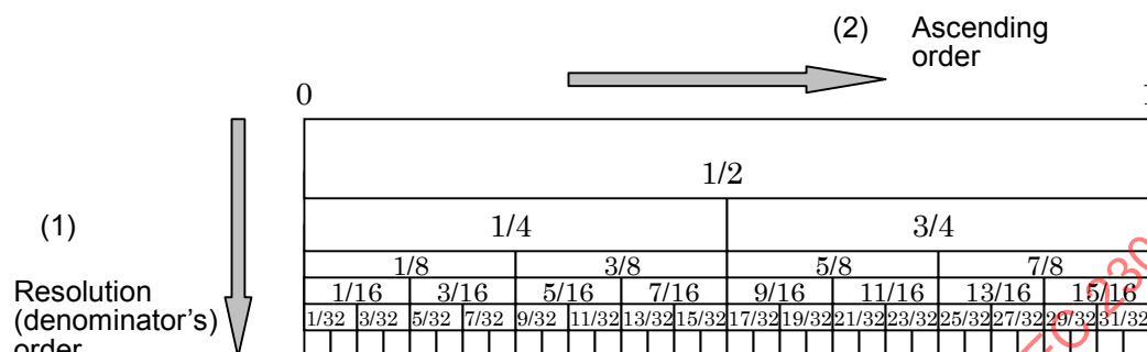
Figure 18 — Order of rational numbers
