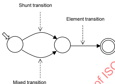
Figure 32 — Example of an element declaration node automaton in case of mixed content model
