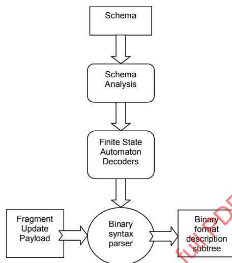
Figure 25 — The complex content decoding process
