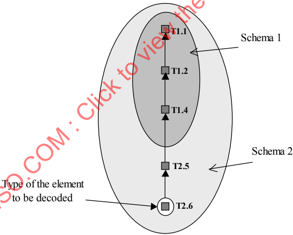
Figure 22 — Example of a type hierarchy defined across versions
