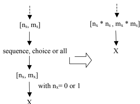
Figure 27 — Group simplification rule
