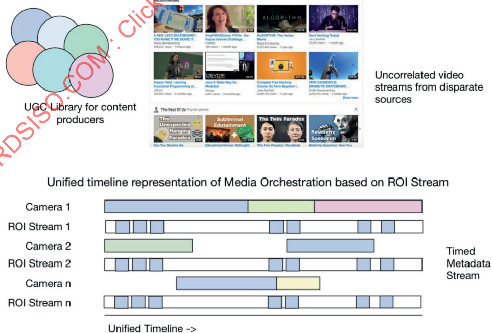
Figure 19 — Timeline representation for media orchestration
