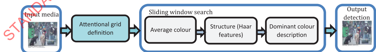
Figure 24 — DROP search process
