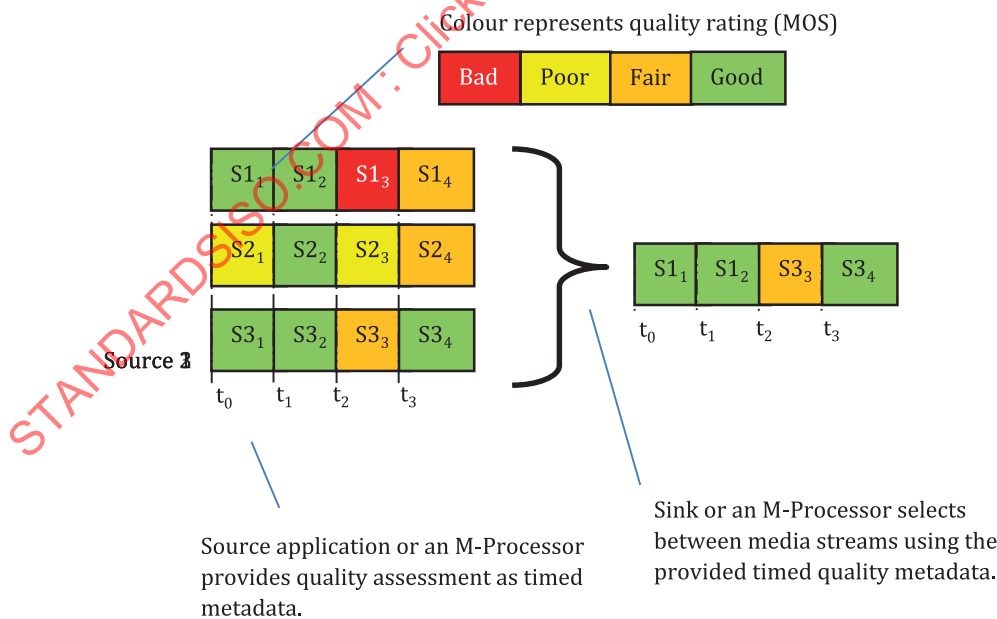
Figure 26 — M-processor selects between sources based on subjective quality
