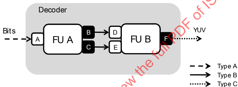
Figure 4 — Three types of connection in an FU network
