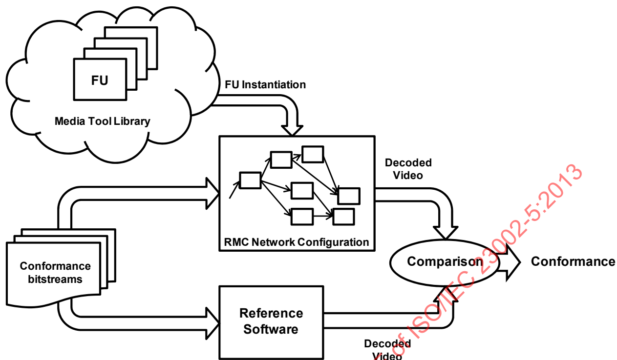
Figure 1 — Concept of RMC decoder level conformance testing
