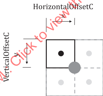
Figure 5 — Location of the top-left chroma sample when ChromaFormatIdc is equal to 1 (4:2:0 chroma format) when Chroma420LocType is equal to 1
