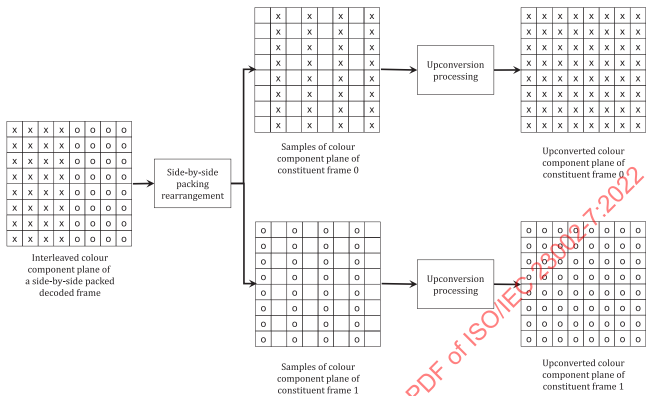
Figure 7 — Flowchart for rearrangement and upconversion of side-by-side packing arrangement with fp_arrangement_type equal to 3, fp_quincunx_sampling_flag equal to 0, ( x, y ) equal to ( 12, 8 ) for constituent frame 0 and ( x, y ) equal to ( 0, 0 ) or ( 4, 8 ) for constituent frame 1
