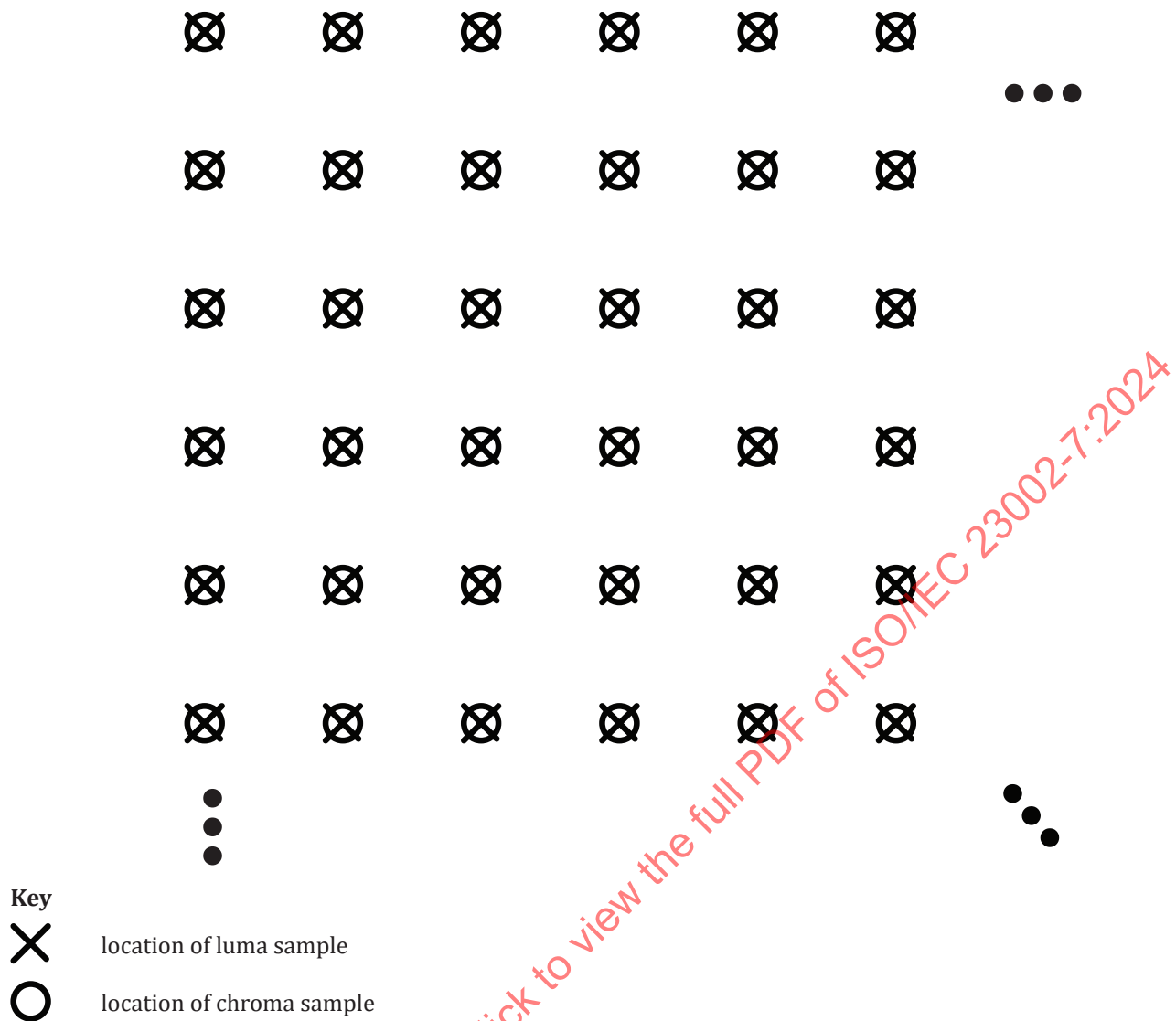
Figure 3 — Nominal vertical and horizontal locations of 4:4:4 luma and chroma samples in a picture
