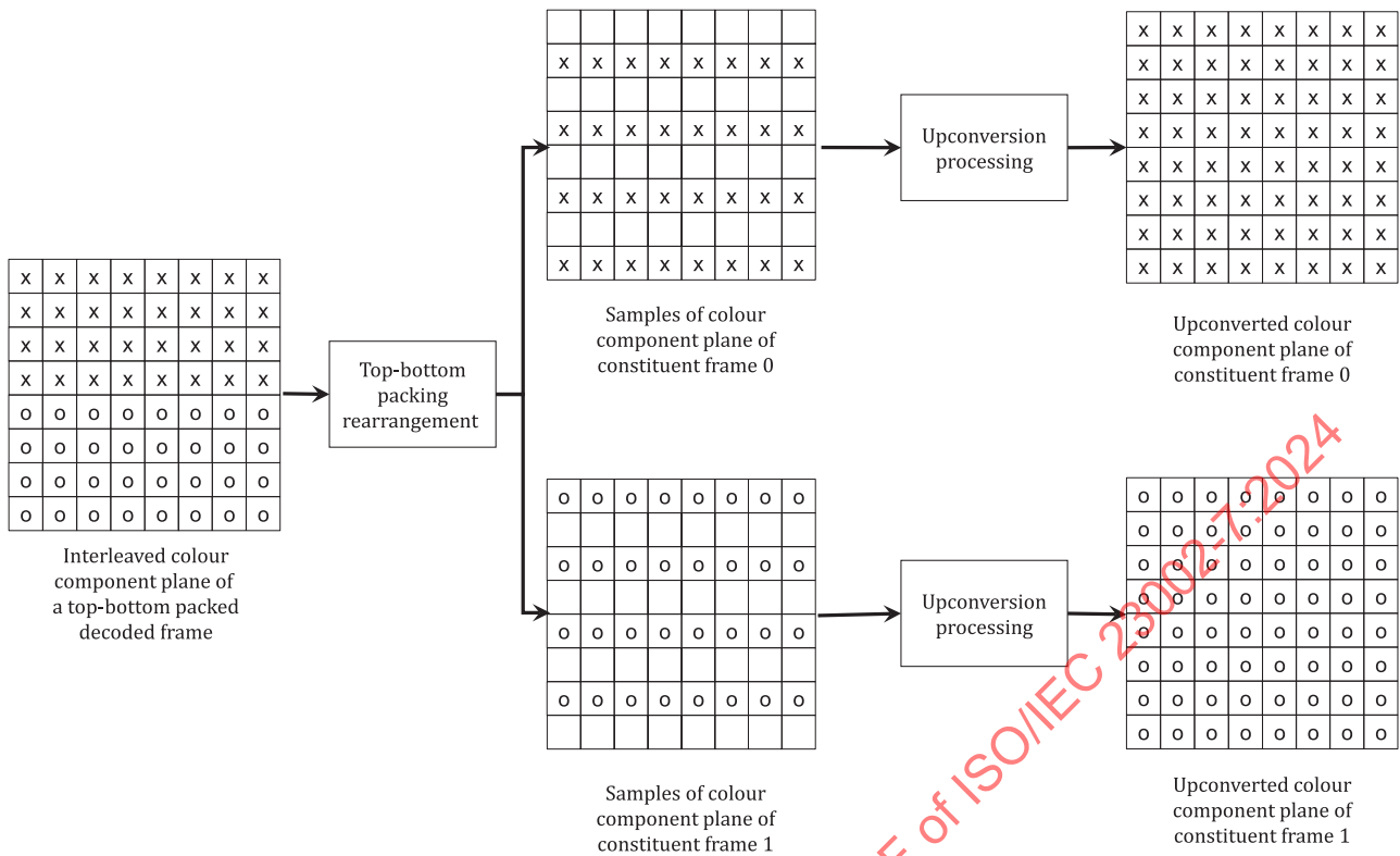
Figure 9 — Flowchart for rearrangement and upconversion of top-bottom packing arrangement with fp\_arrangement\_type equal to 4, fp\_quincunx\_sampling\_flag equal to 0, (x, y) equal to ( 8, 12 ) for constituent frame 0 and (x, y) equal to ( 0, 0 ) or ( 8, 4 ) for constituent frame 1
