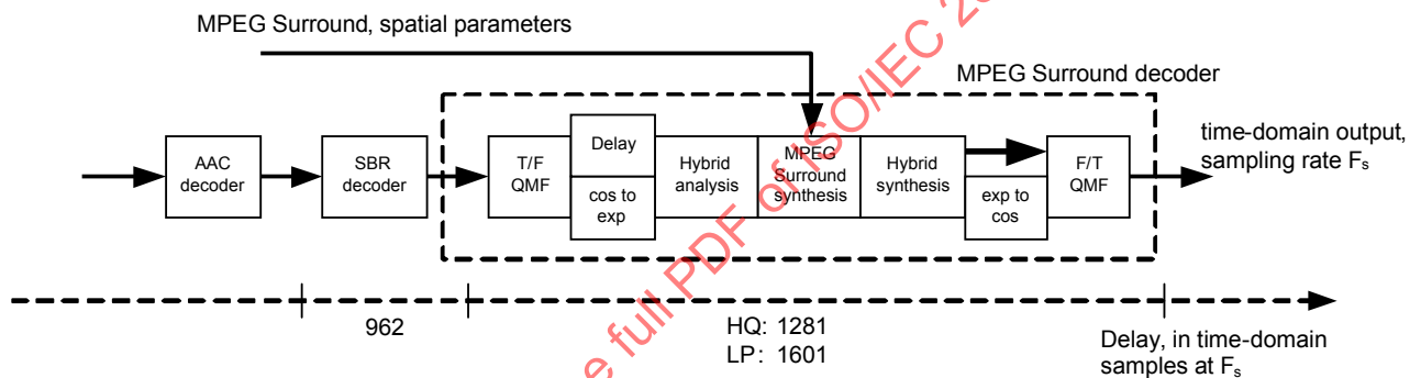
Figure 11, where the HE-AAC decoder comprises AAC and SBR decoding.
