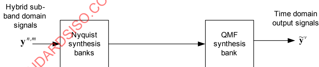
Figure 21 — Time/frequency transforms in MPEG Surround, hybrid QMF synthesis bank
