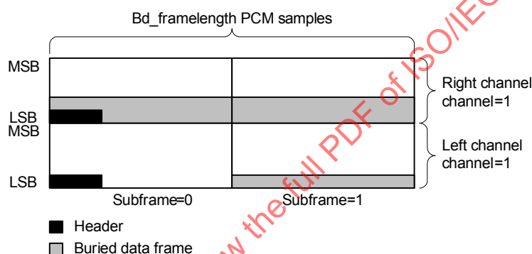
Figure 56 — Example buried data frame-structure with header.
