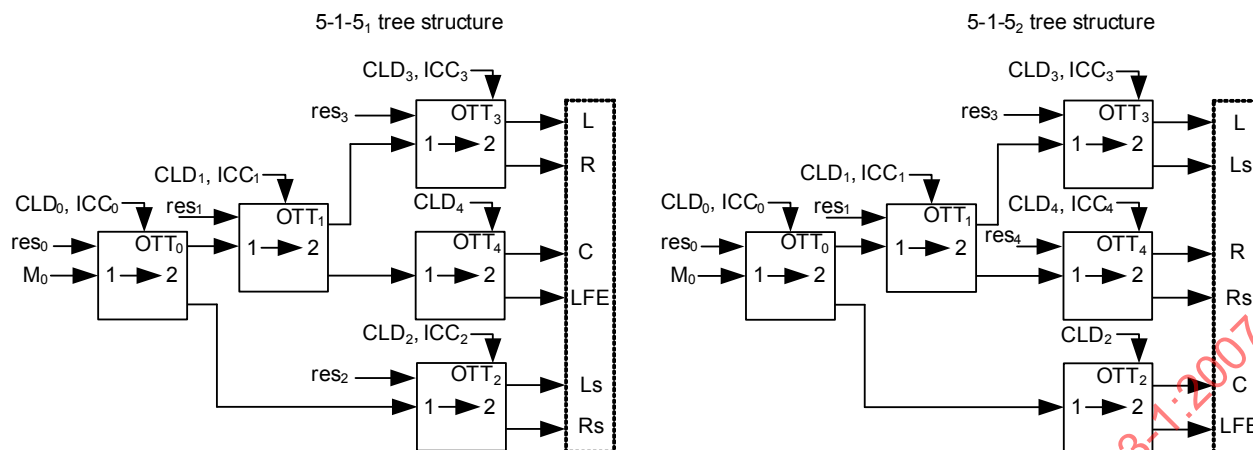
Figure 23 — Tree structure view of the spatial audio processing for the 5-1-5 configurations
