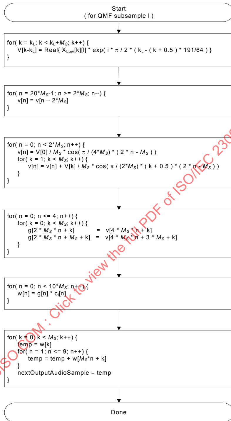
Figure 10 — Flowchart of real-valued sub-sampled M S -ch synthesis QMF bank
