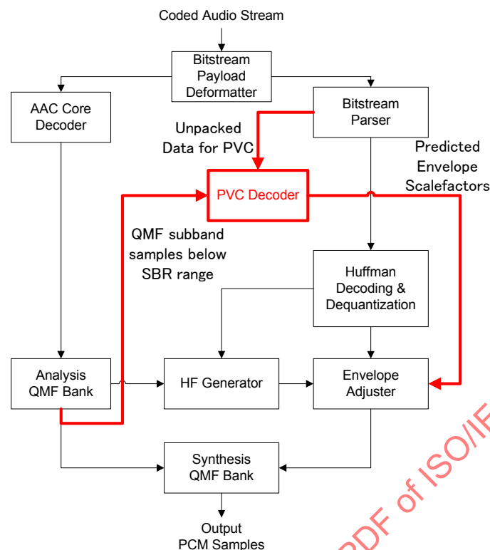
Figure 17 — Block diagram of the decoder including PVC decoder
