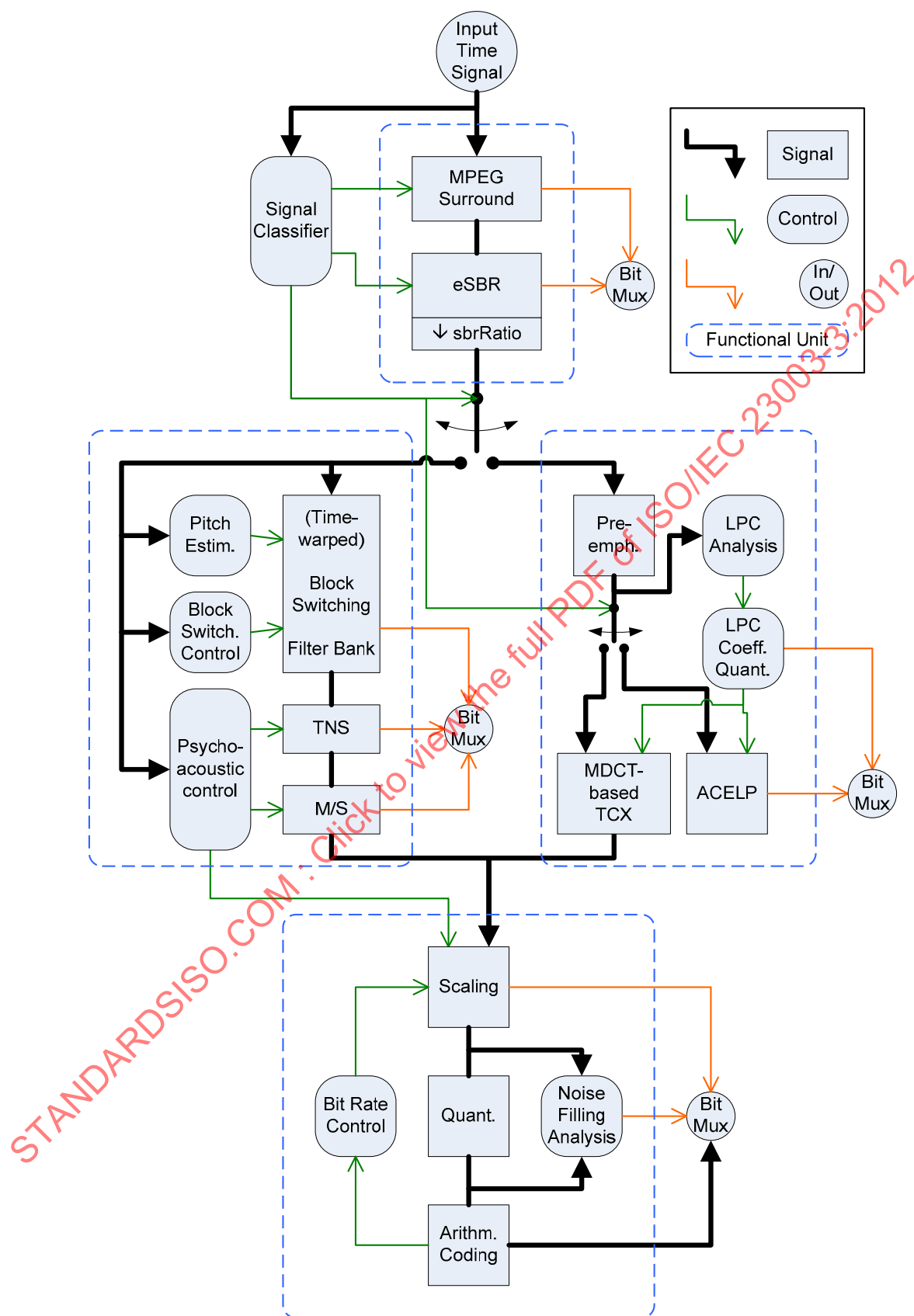
Figure B.1 — Block diagram of the USAC encoder
