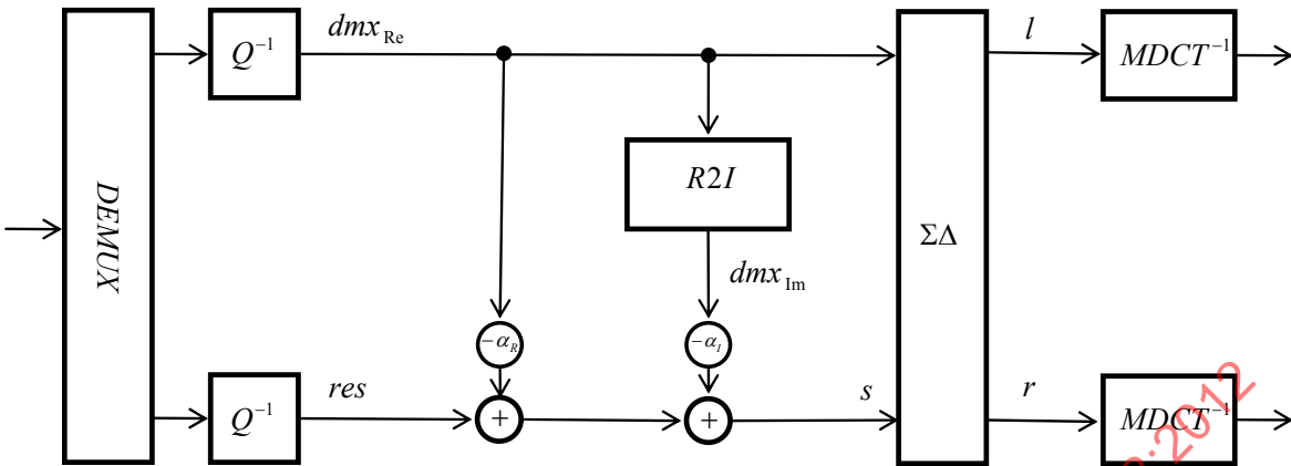
Figure 19 — Block diagram of the decoder with complex stereo prediction
