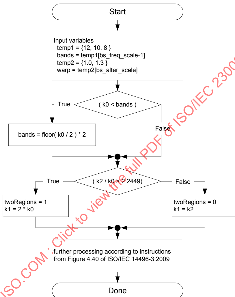
Figure 12 — Flowchart calculation of f_{Master} for 4:1 system when bs\_freq\_scale > 0
