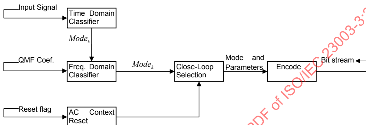
Figure B.2 — Structure of Classification based ACELP-TCX Selection
