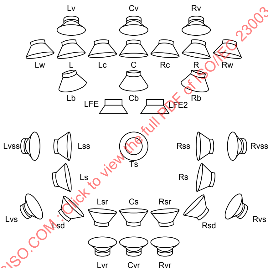
Figure 2 — Loudspeaker positions
