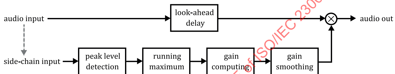
Figure AMD1.3 — Time domain peak limiter design of parametricDrcType==0x1
