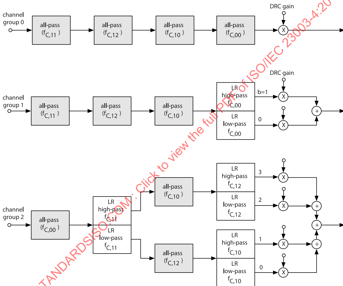
Figure 7 — Example of phase adjustments for time-domain multiband DRC with different DRC bands for each channel group
