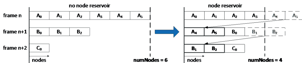
Figure 5 — Illustration of node reservoir mechanism: A_x , B_x , and C_x are nodes regularly transmitted in DRC frame n , n+1 , and n+2 , respectively (left). When the node reservoir is used, some nodes (bold) are transmitted with a delay of one frame (right)
