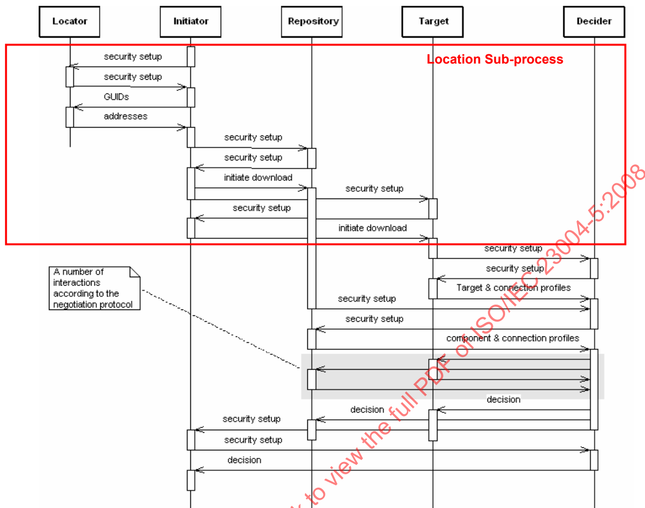
Figure 5 — Sequence diagram highlighting the location sub-process
