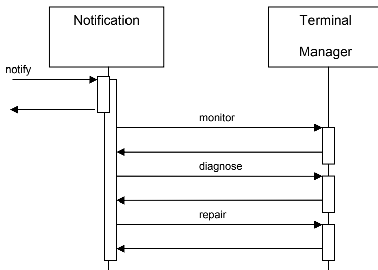
Figure 11 — Notification Message Sequence Chart
