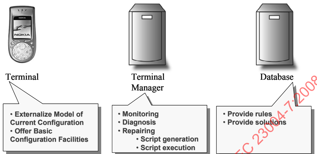
Figure 7 — Responsibilities of System Integrity Management roles
