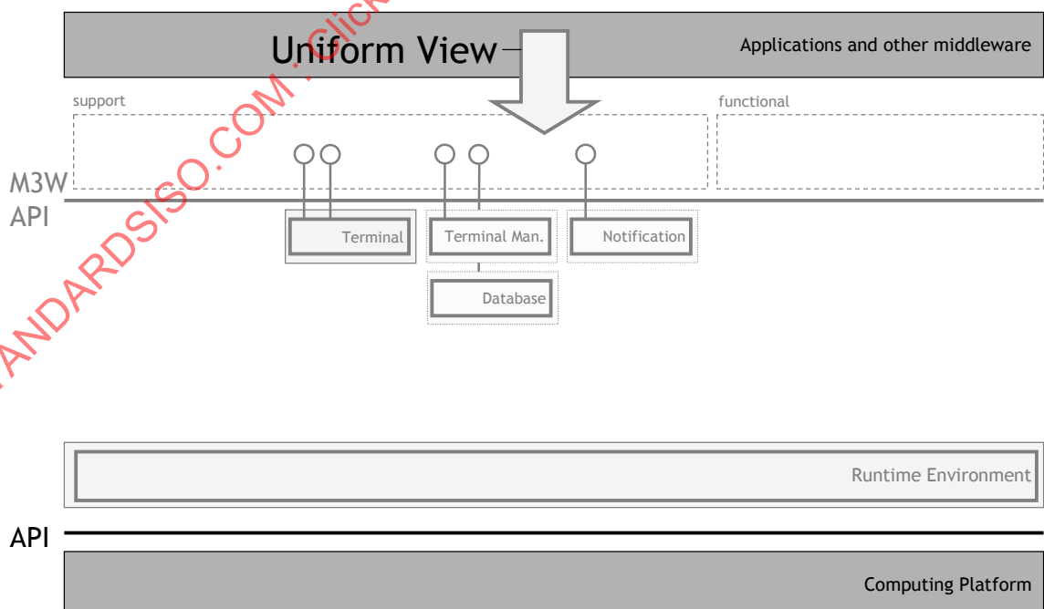
Figure 1 — M3W Integrity Management API
