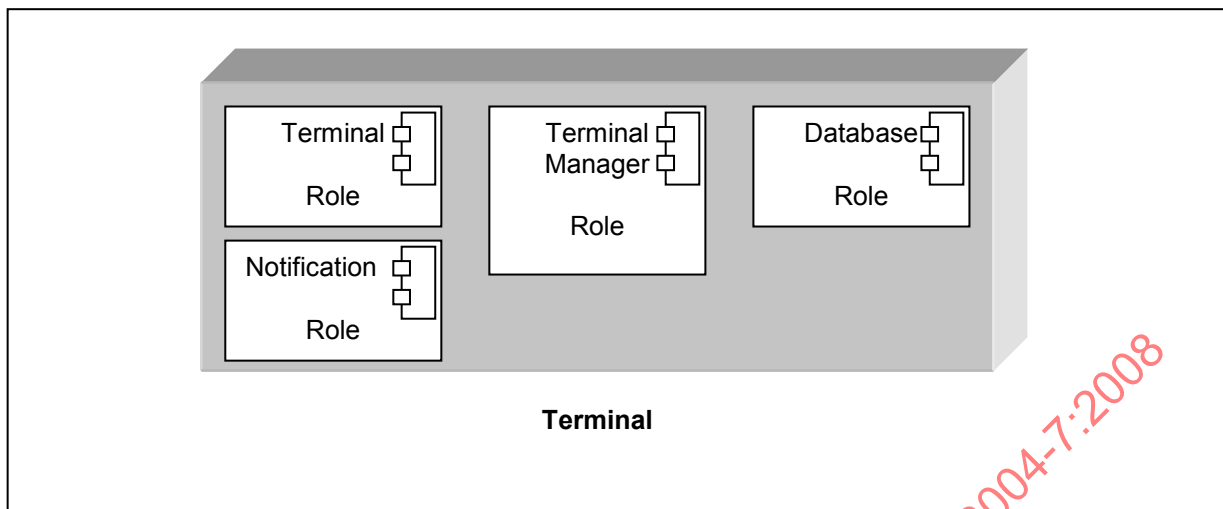
Figure 12 — Deployment - Terminal
