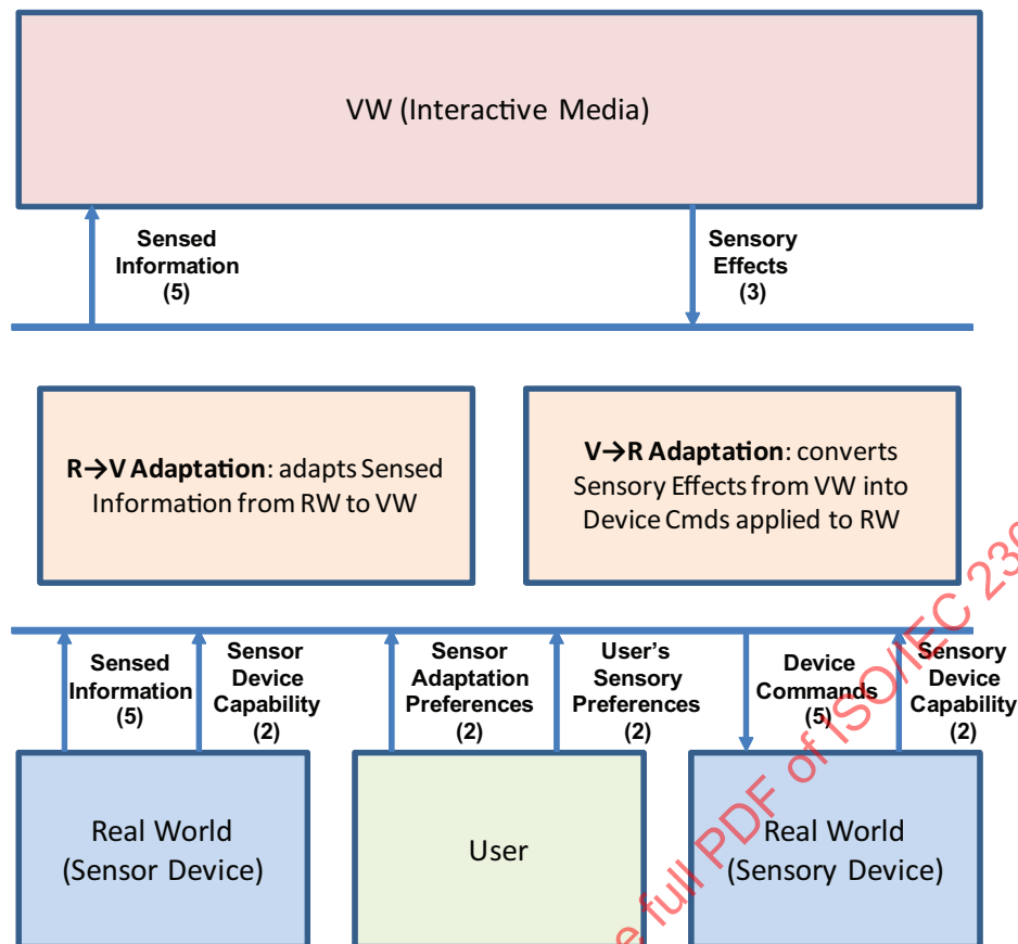
Figure 35 — (Possible) System Architecture for Interactive haptic sensible media
