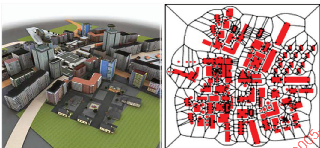
Figure 24 — Example of a virtual test city environment and its footprints and corridor map
