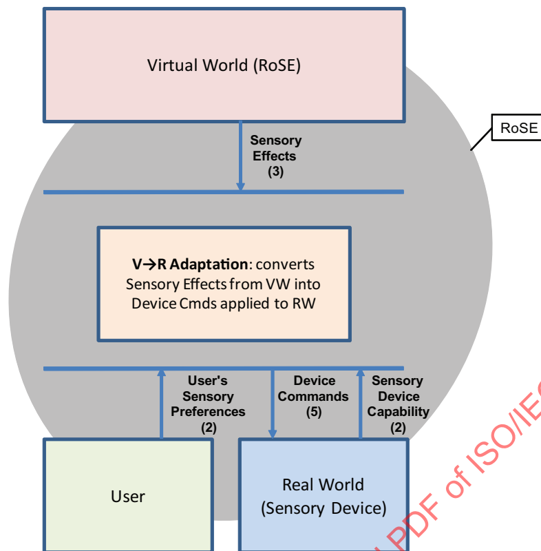
Figure 5 — RoSE System Architecture
