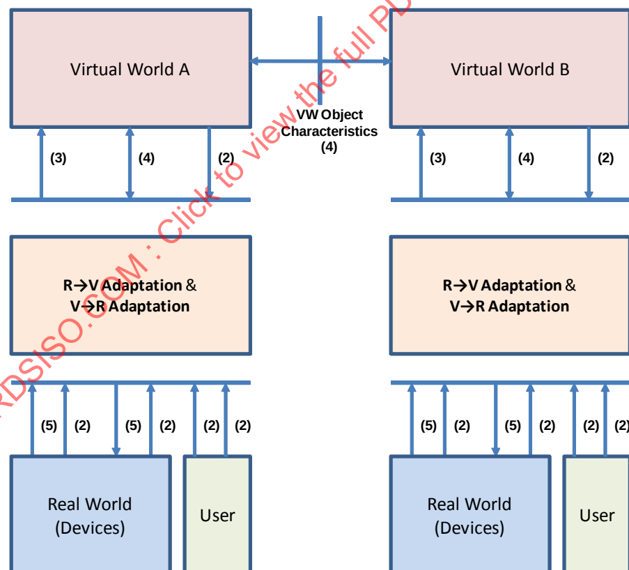
Figure 4 — (Possible) System Architecture for (bidirectional) exchange of information between virtual worlds
