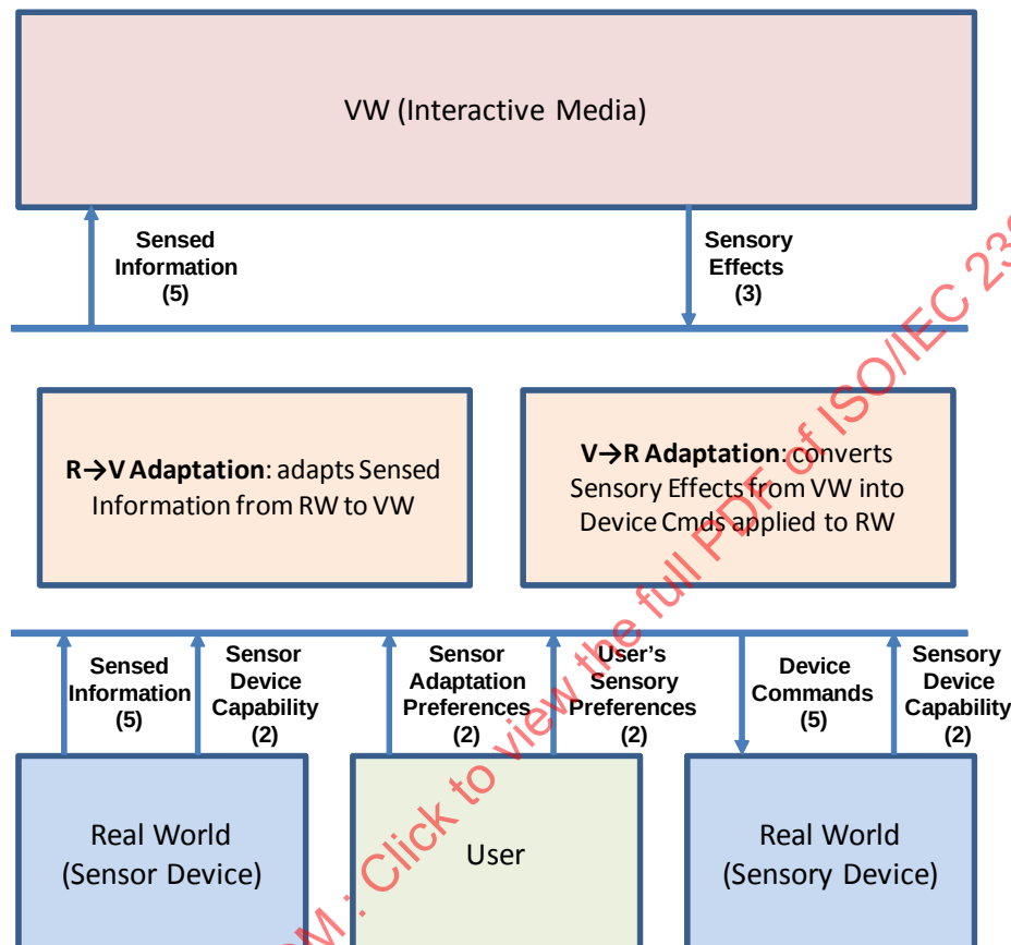
Figure 35 — (Possible) System Architecture for Interactive haptic sensible media
