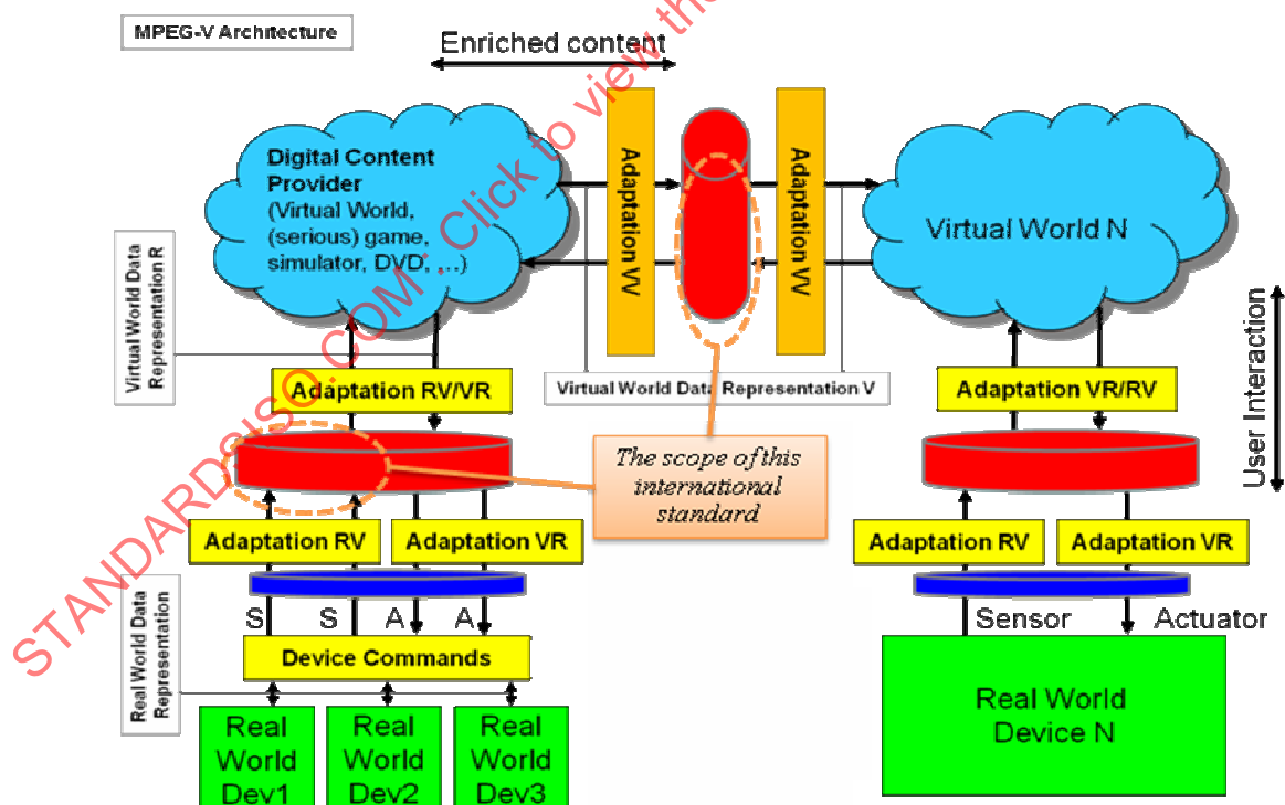
Figure 1 – System Architecture
