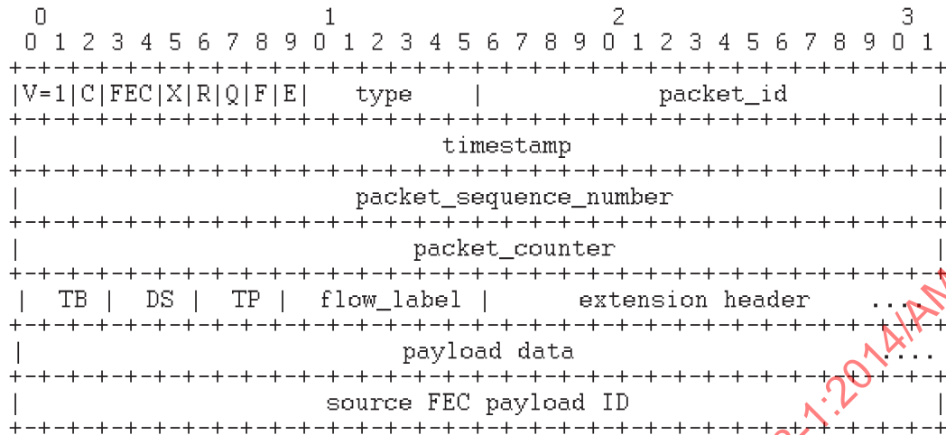
Figure — AMD1.3 — MMTP packet header, payload and footer
