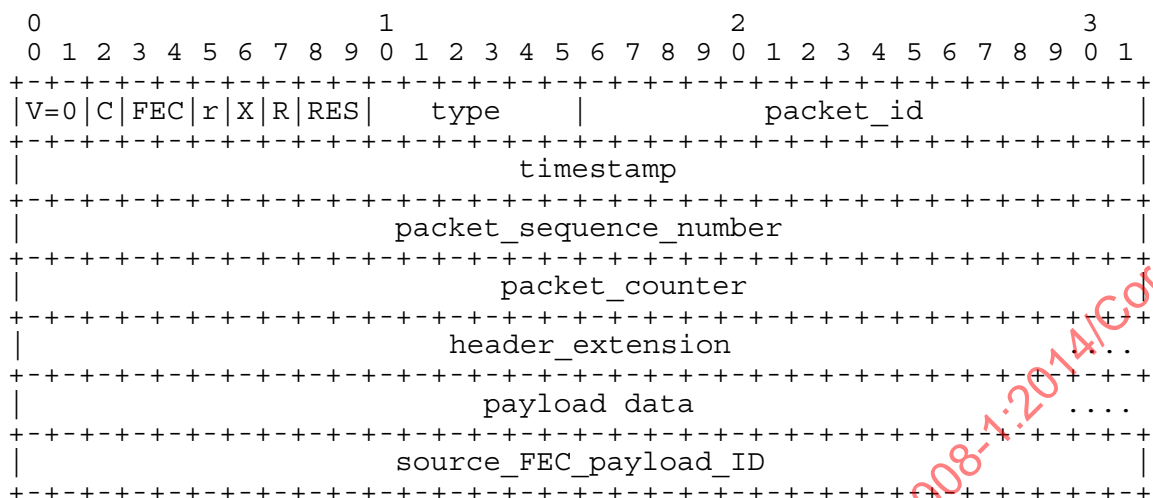
Figure 1 — Structure of MMTP packet
