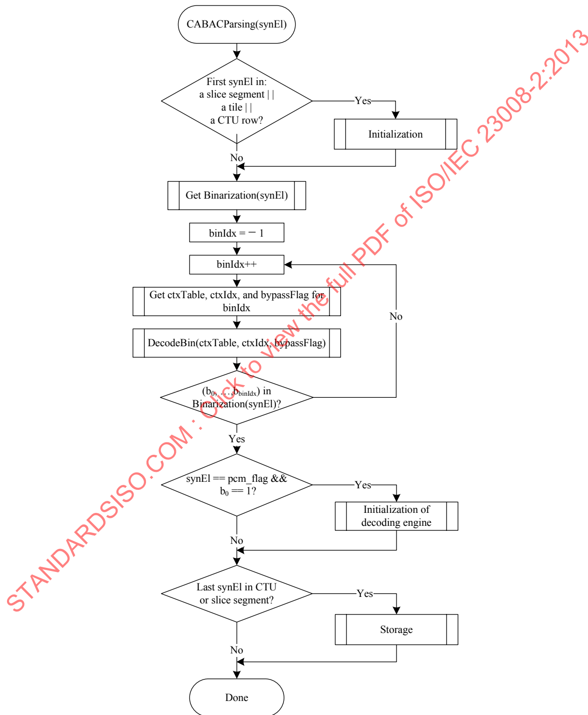
Figure 9-1 – Illustration of CABAC parsing process for a syntax element synEl (informative)
