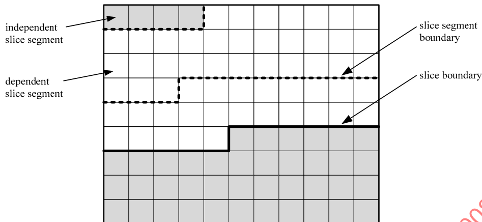
Figure 6-4 – A picture with 11 by 9 luma coding tree blocks that is partitioned into two slices, the first of which is partitioned into three slice segments (informative)
