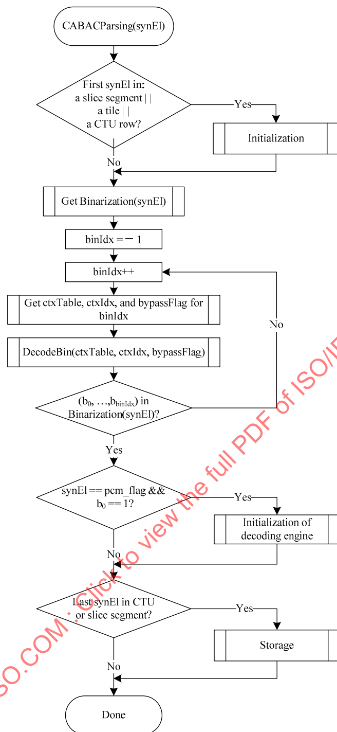
Figure 9-1 – Illustration of CABAC parsing process for a syntax element synEl (informative)
