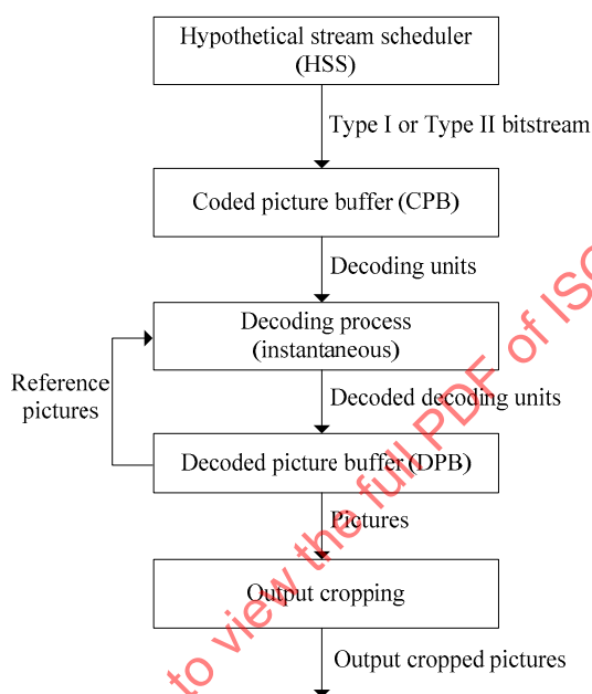
Figure C.2 – HRD buffer model
