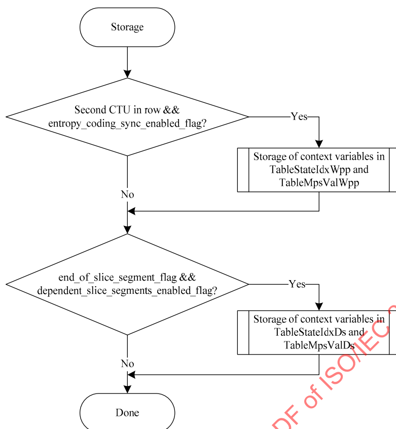
Figure 9-4 – Illustration of CABAC storage process (informative)
