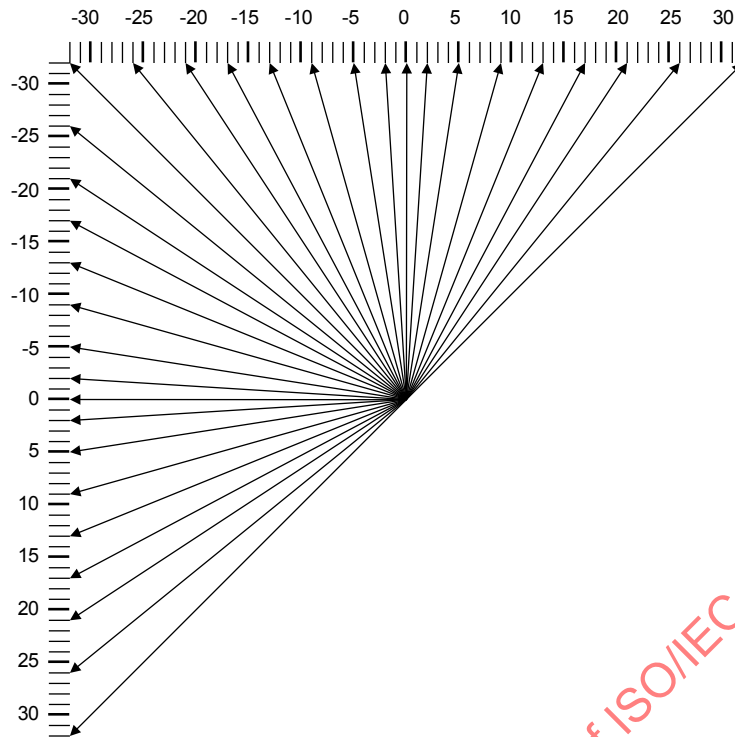
Figure 8-2 — Intra prediction angle definition (informative)
