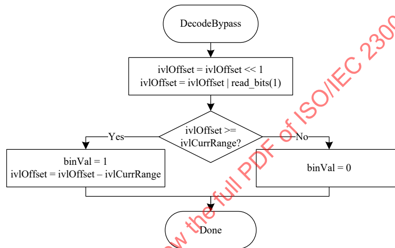
Figure 9-8 — Flowchart of bypass decoding process
