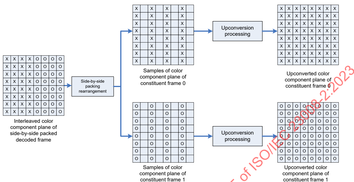
Figure D.4 — Rearrangement and upconversion of side-by-side packing arrangement with frame_packing_arrangement_type equal to 3, quincunx_sampling_flag equal to 0, and (x, y) equal to (0, 0) or (4, 8) for both constituent frames
