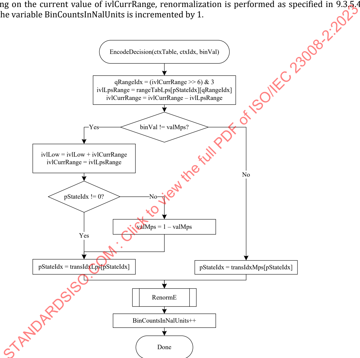
Figure 9-10 — Flowchart for encoding a decision
