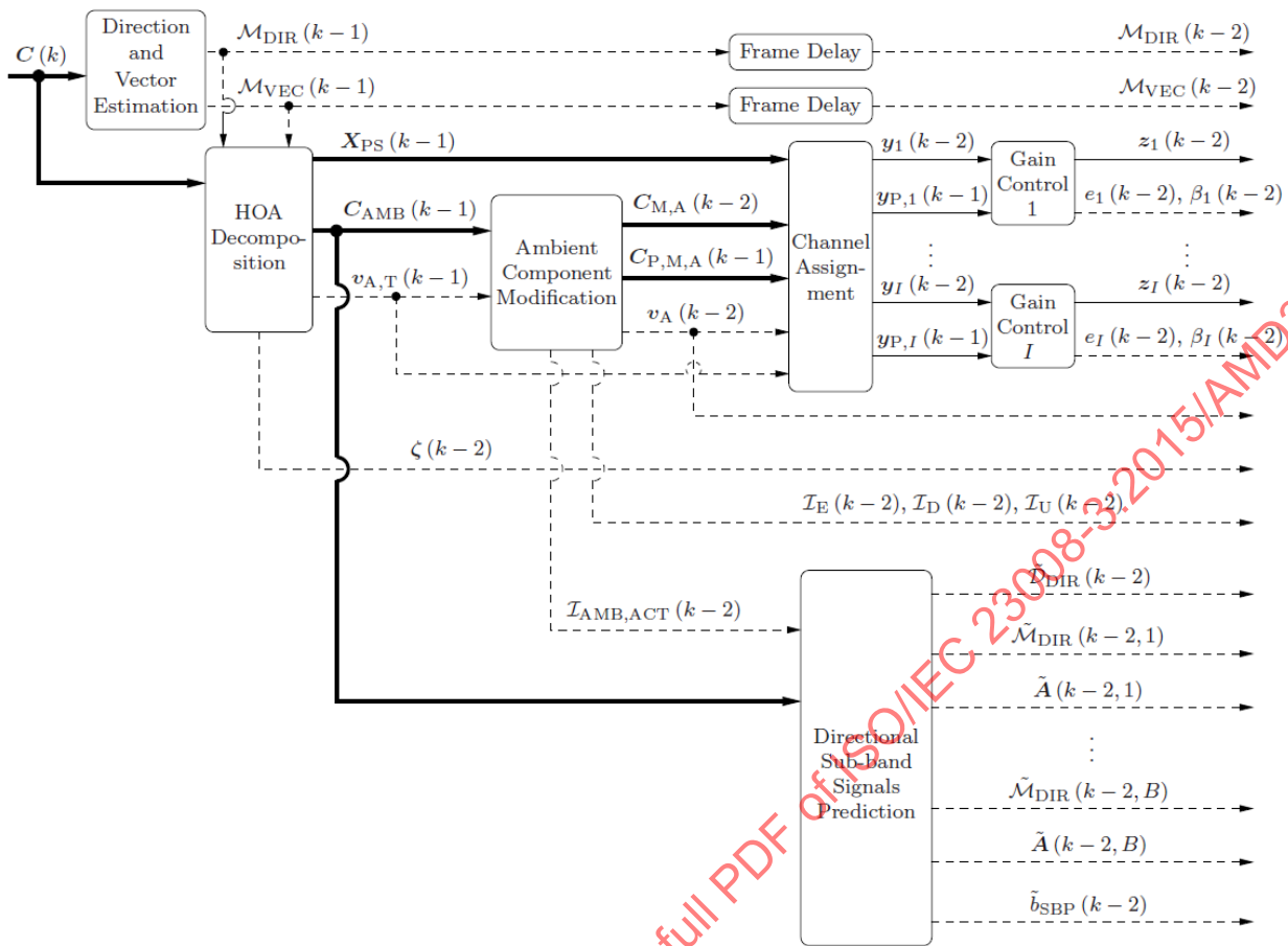
Figure AMD1.4 — Architecture of spatial HOA encoder (part 1)
