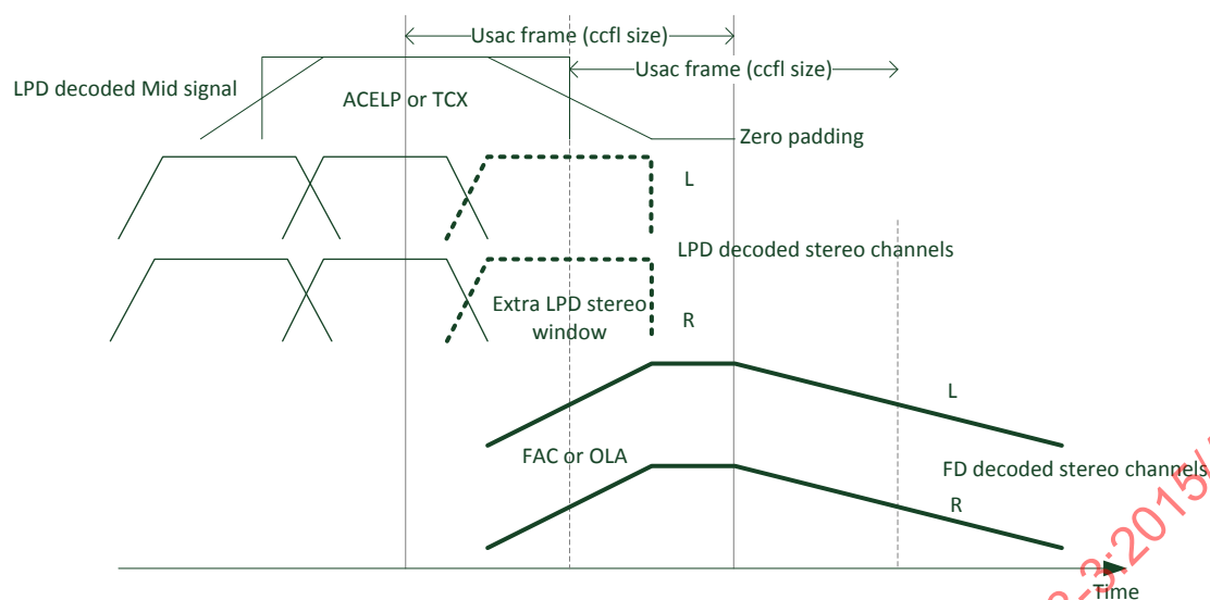
Figure AMD3.2 — Schematic representation of the transition from LPD to FD mode with LPD stereo.
