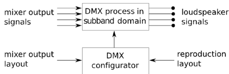
Figure FC.1 — Main building blocks of the low complexity generic format converter
