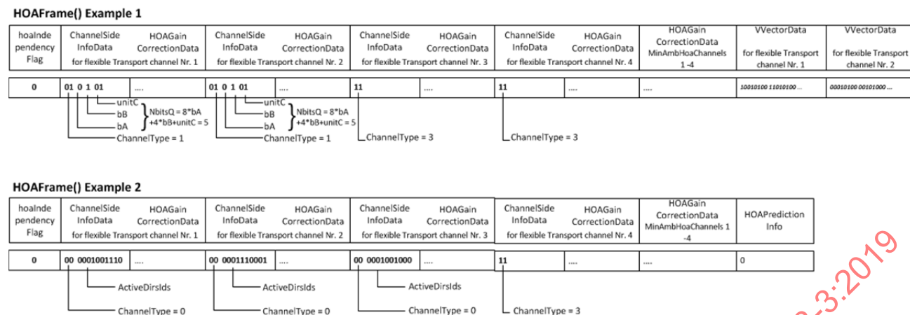
Figure 58 — Two examples for HOAFrame()
