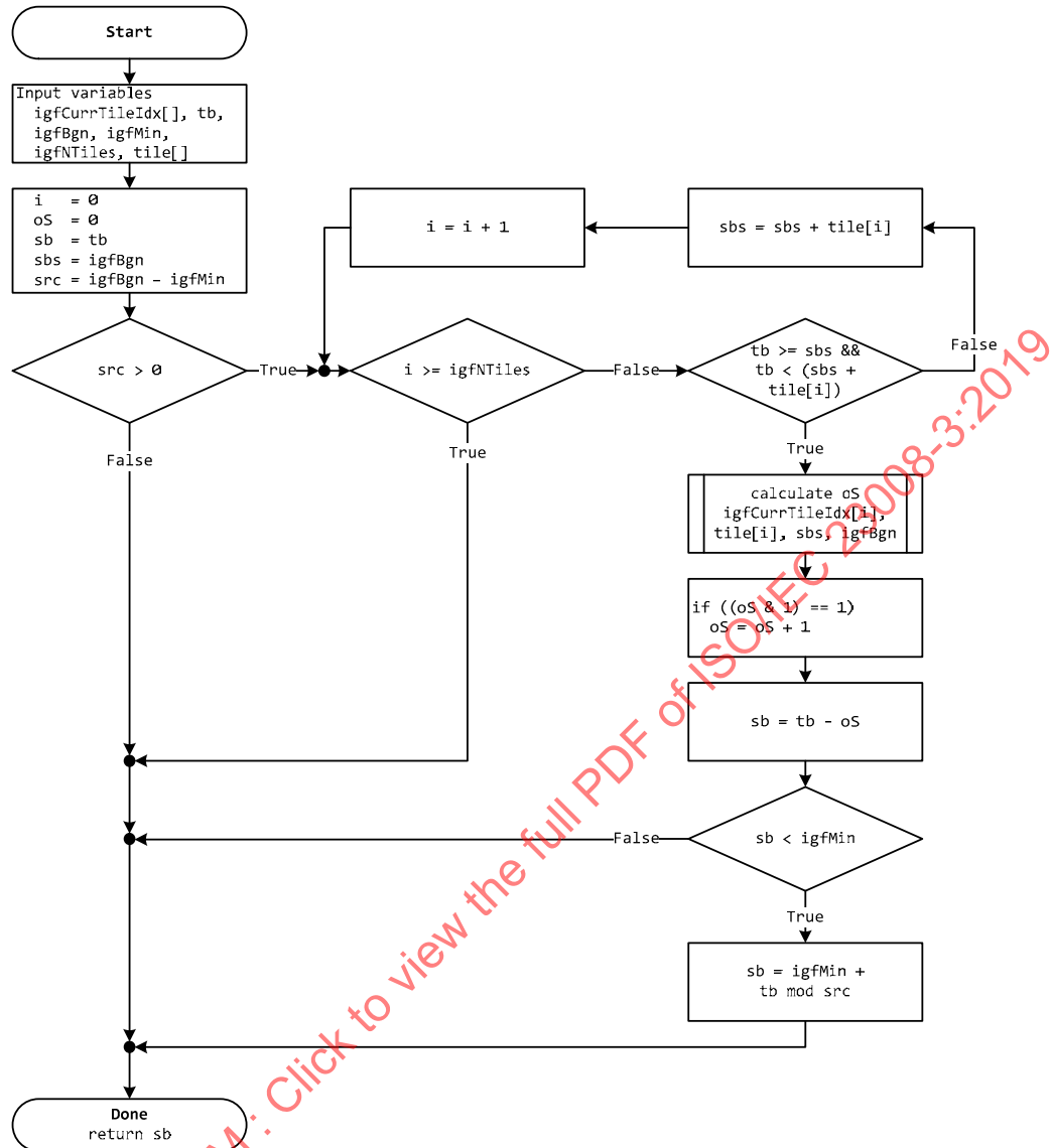
Figure 16 — Flowchart for computing a source subband sb
