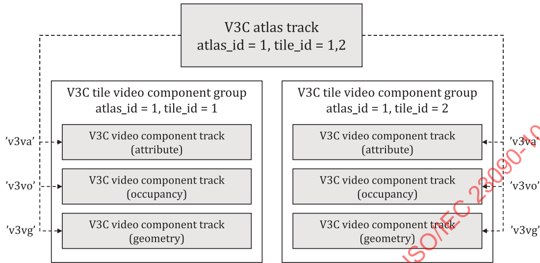
Figure 4 — Example of V3C tile video component track grouping
