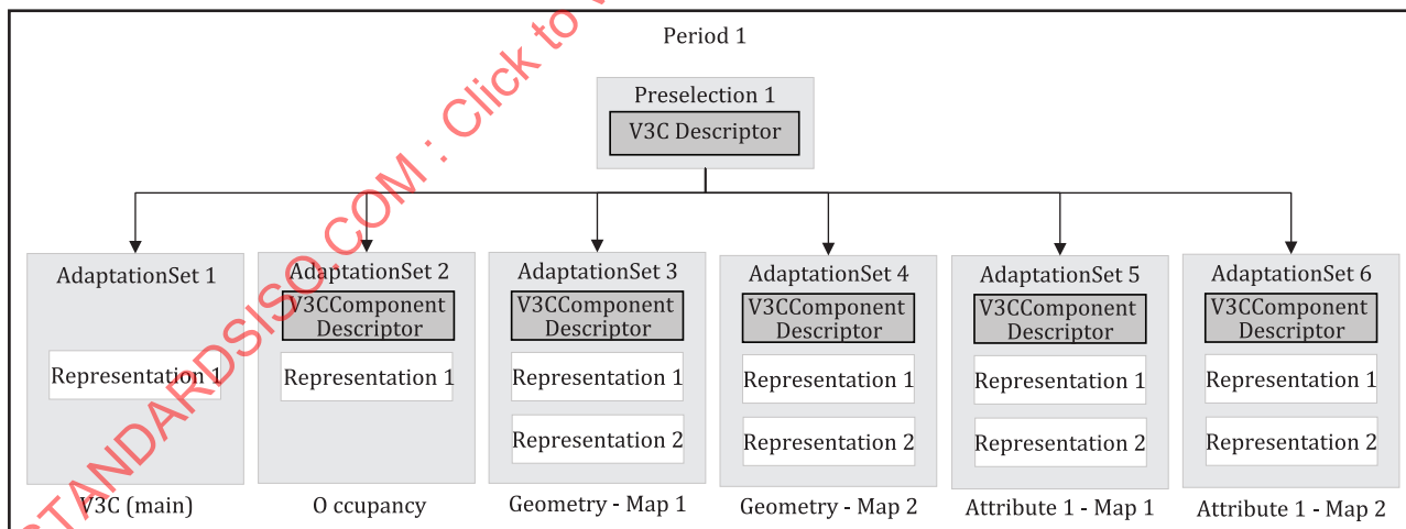
Figure 5 — Grouping V3C components in an MPD using Preselections
