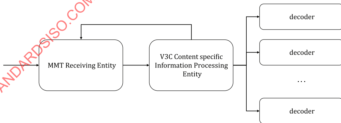
Figure 6 — Conceptual architecture of the client receiving V3C Content with MMT
