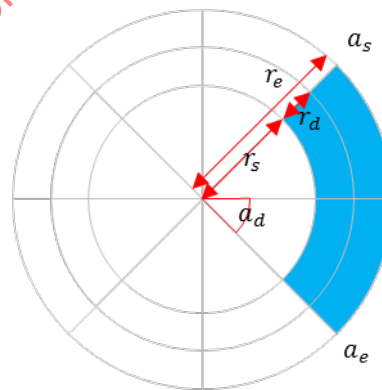
Figure 15 — Illustration of parameters regarding local FOV
