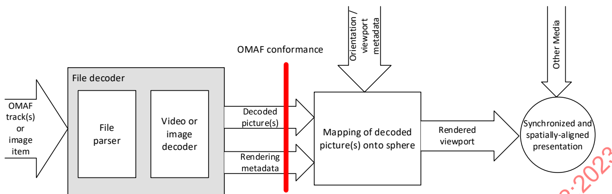
Figure 4 — Conformance points for OMAF video and image media profiles
