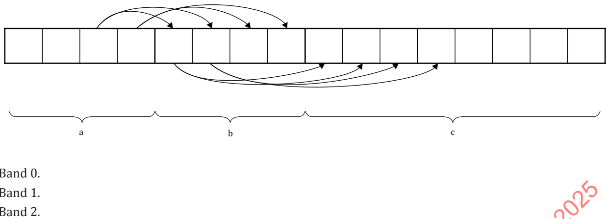
Figure 34 — SPIHT spatial orientation tree
