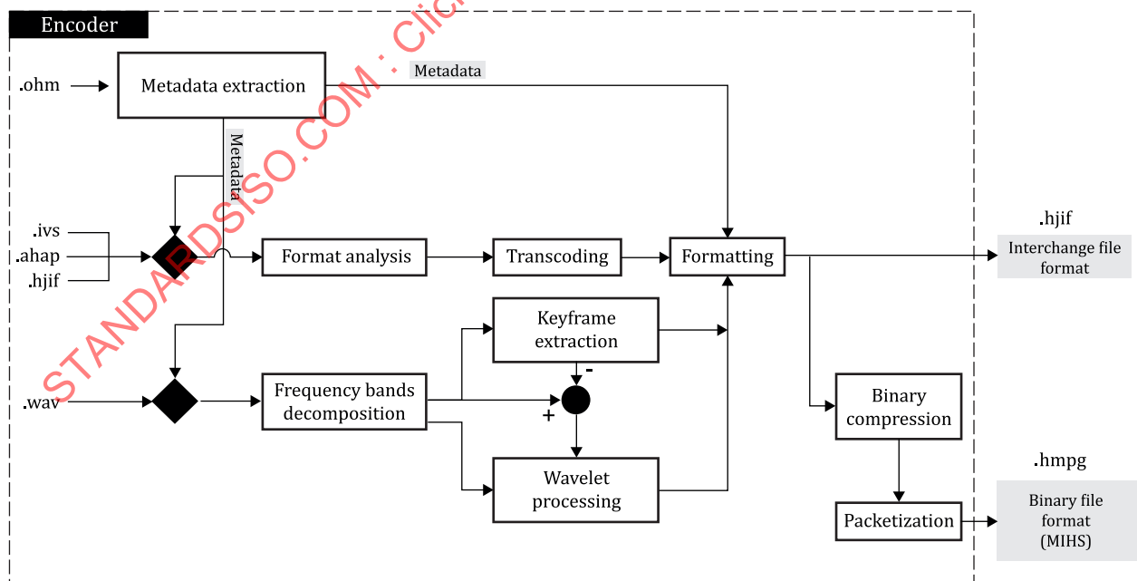
Figure 30 — Encoder architecture
