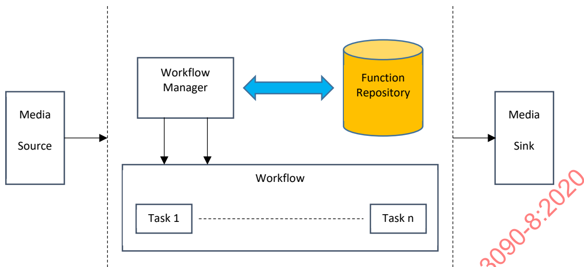
Figure 2 — Workflow manager interworking with function repository
