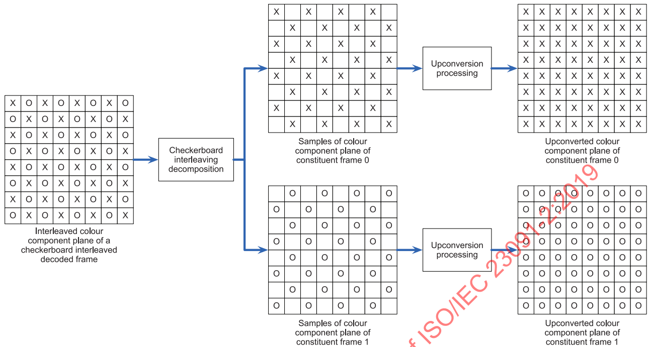
Figure 2 — Rearrangement and upconversion of checkerboard interleaving (VideoFramePackingType equal to 0)
