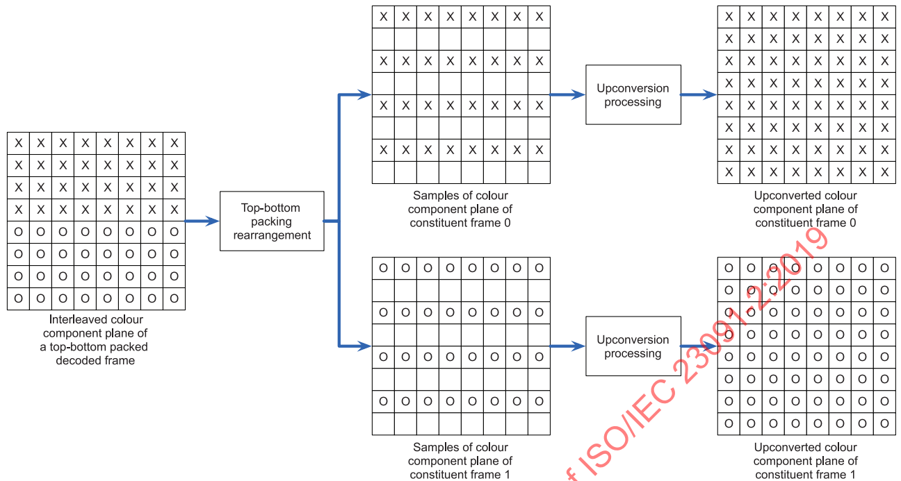
Figure 6 — Rearrangement and upconversion of top-bottom packing arrangement (VideoFramePackingType equal to 4 with QuincunxSamplingFlag equal to 0)
