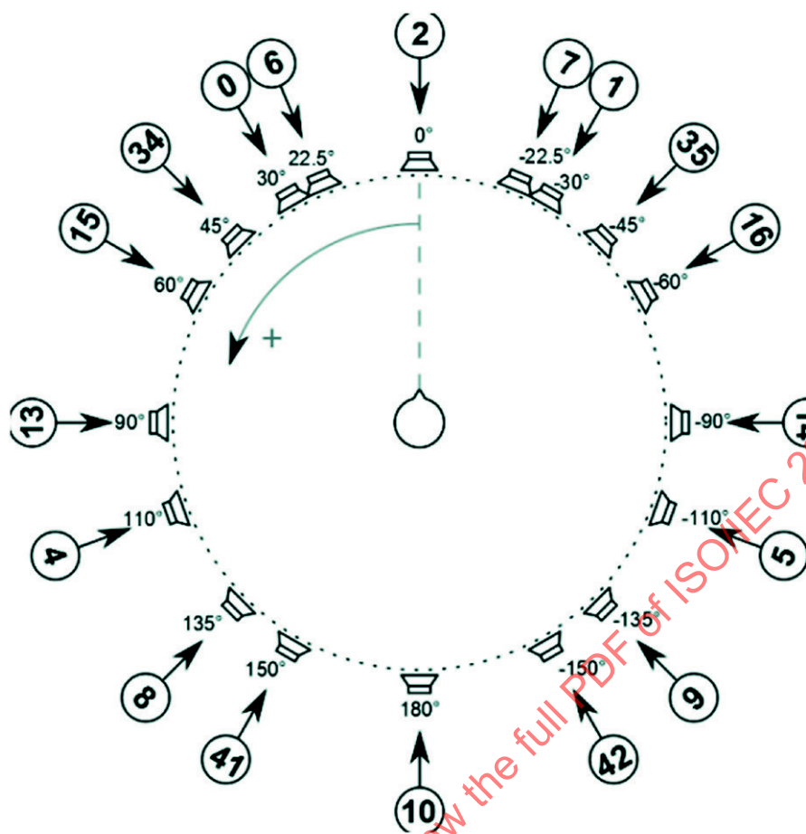
Figure 4 — Loudspeaker positions, mid layer
