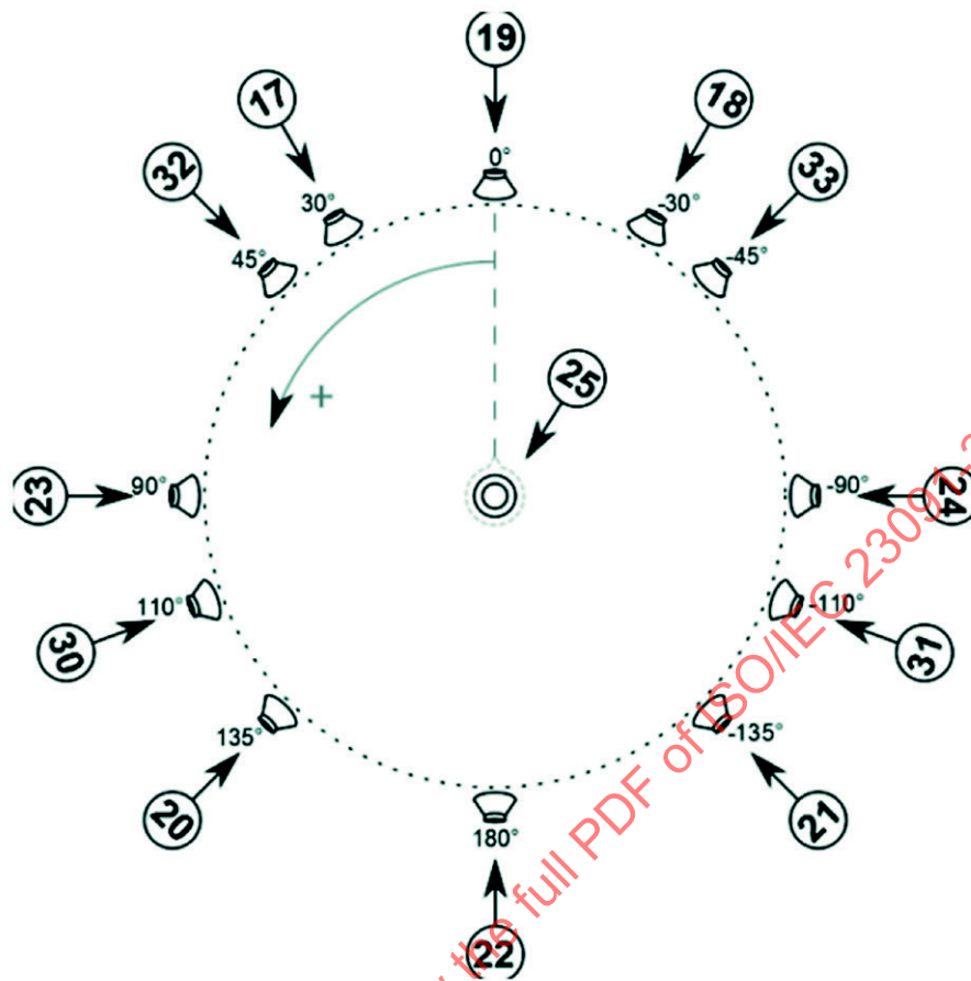
Figure 3 — Loudspeaker positions, upper layer [index 25 indicates the loudspeaker directly above the listener, sometimes referred to as the "voice of god (VoG)" loudspeaker]
