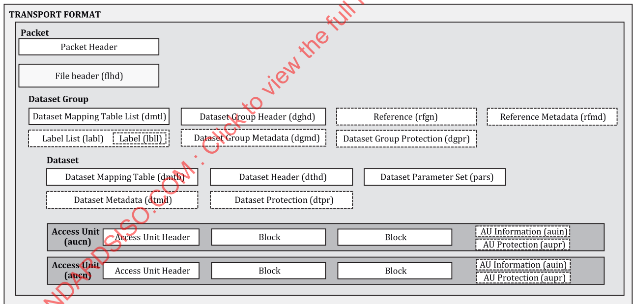
Figure 5 — Data structures hierarchy for transport
