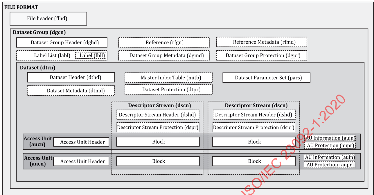
Figure 4 — Data structures hierarchy for storage
