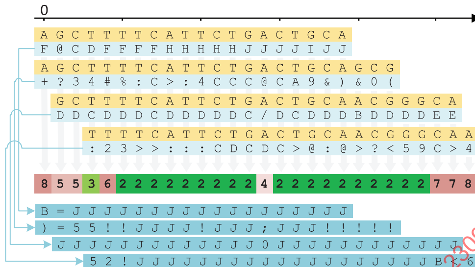
Figure 6 — Relationship between sequencing reads, quality values, reconstructed quality values, and genomic positions
