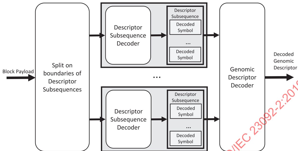
Figure 7 — Block payload parsing process
