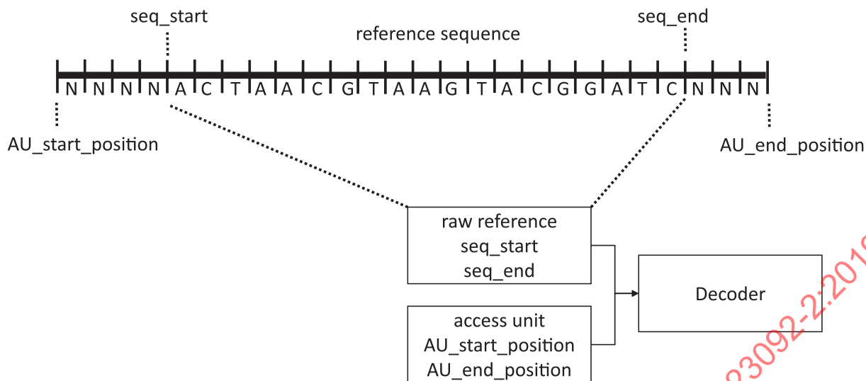
Figure 5 — Padding process for a reference sequence
