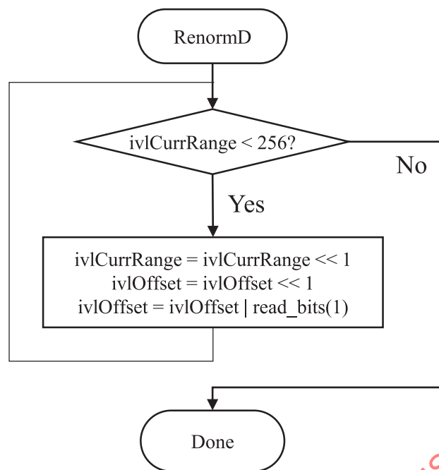
Figure 11 — Flowchart of renormalization
