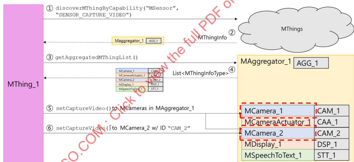
Figure 5 – Process of activating setCaptureVideo() to cameras in an MAggregator
