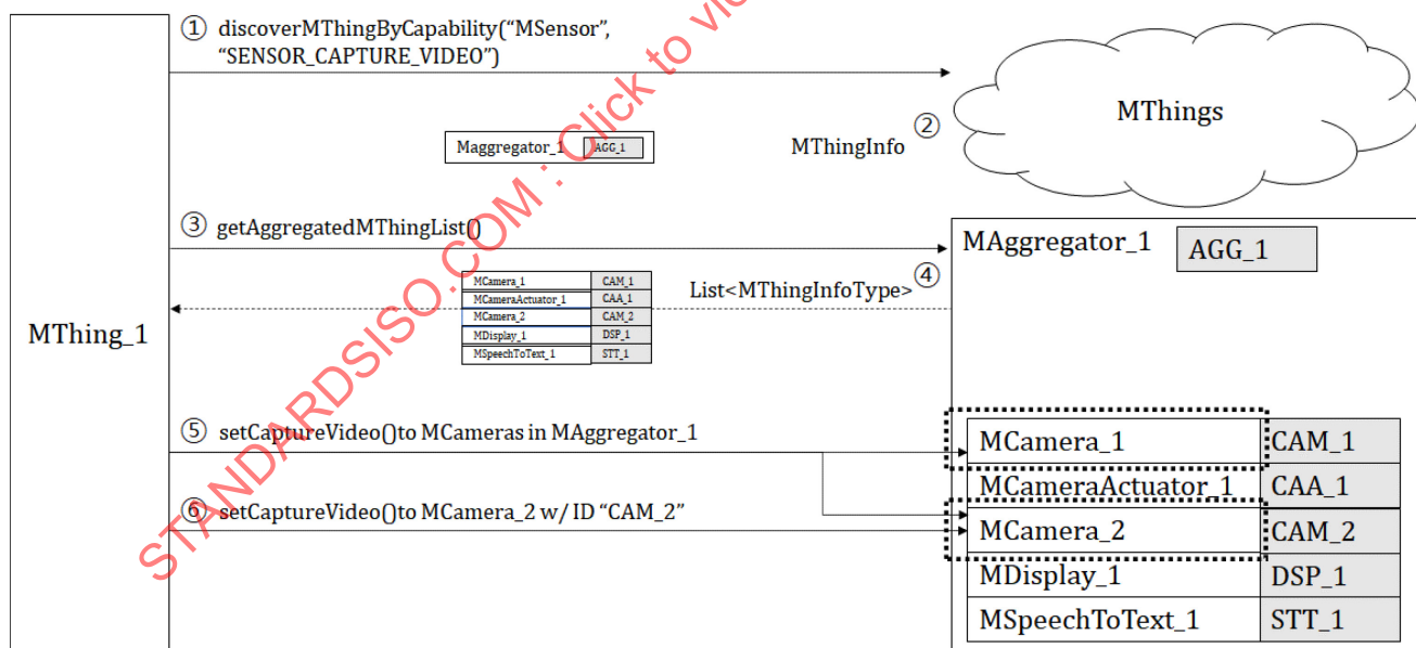
Figure 5 – Process of activating setCaptureVideo() to cameras in a MAggregator
