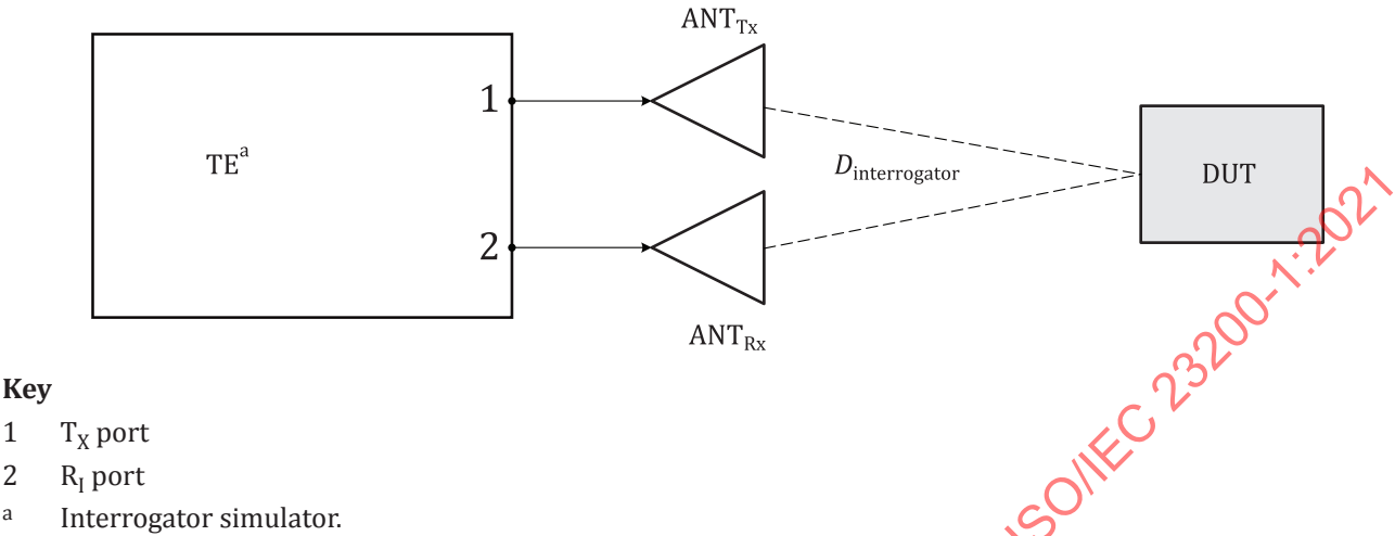
Figure 1 — Bistatic test setup
