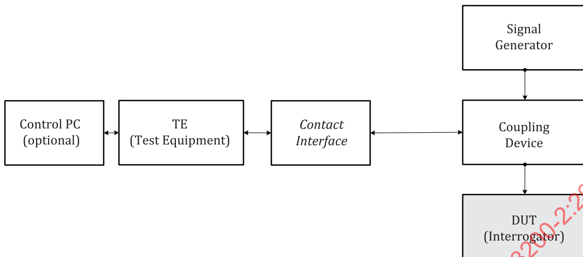
Figure 4 — Contact test setup for rejection measurement
