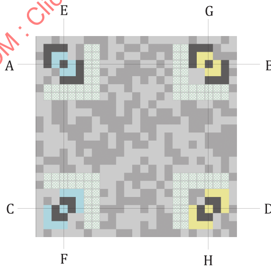
Figure 19 — Finder patterns and guidelines
