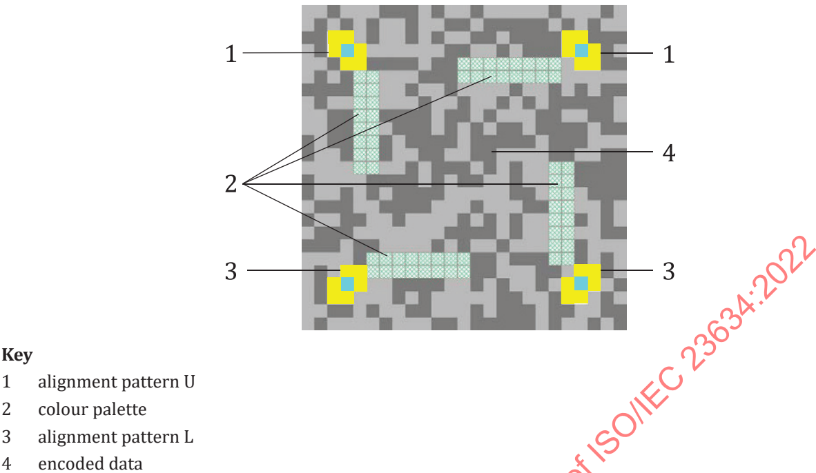
Figure 3 — Structure of square secondary symbol
