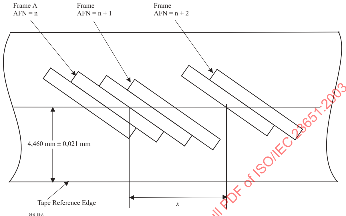
Figure 48 - Tolerance on seamless appending
