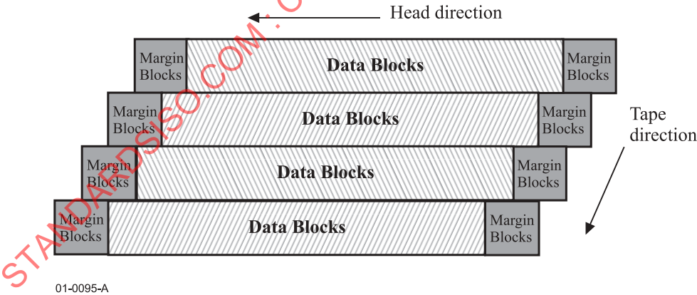
Figure 41 – Format of tracks
