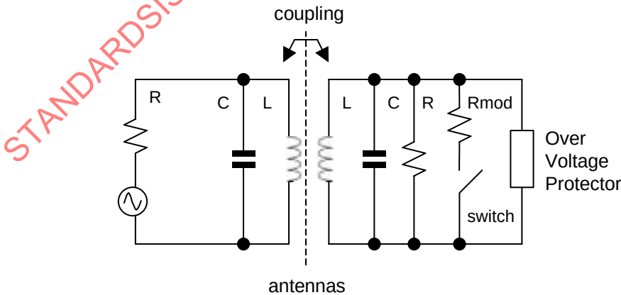
Figure 54 – AIT RMIC interface network
