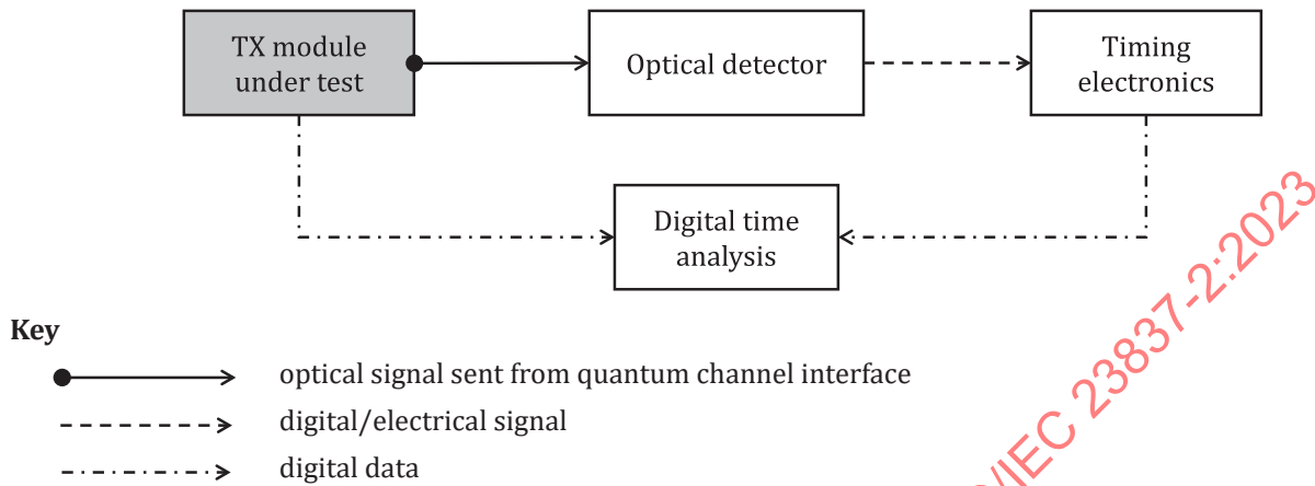
Figure 8 — Schematic of the setup for testing the independence of the intensities of optical pulses
