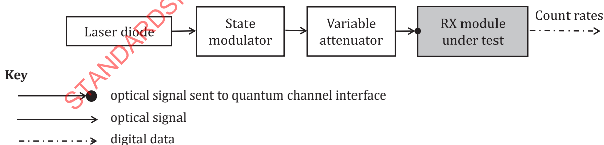
Figure 21 — Setup for testing the temporal profile of the detection efficiency for SPDs
