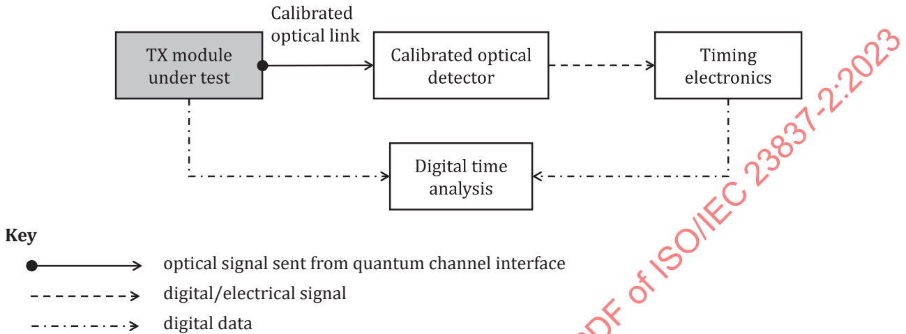
Figure 7 — Schematic of the setup for testing the mean photon number and stability of optical pulses
