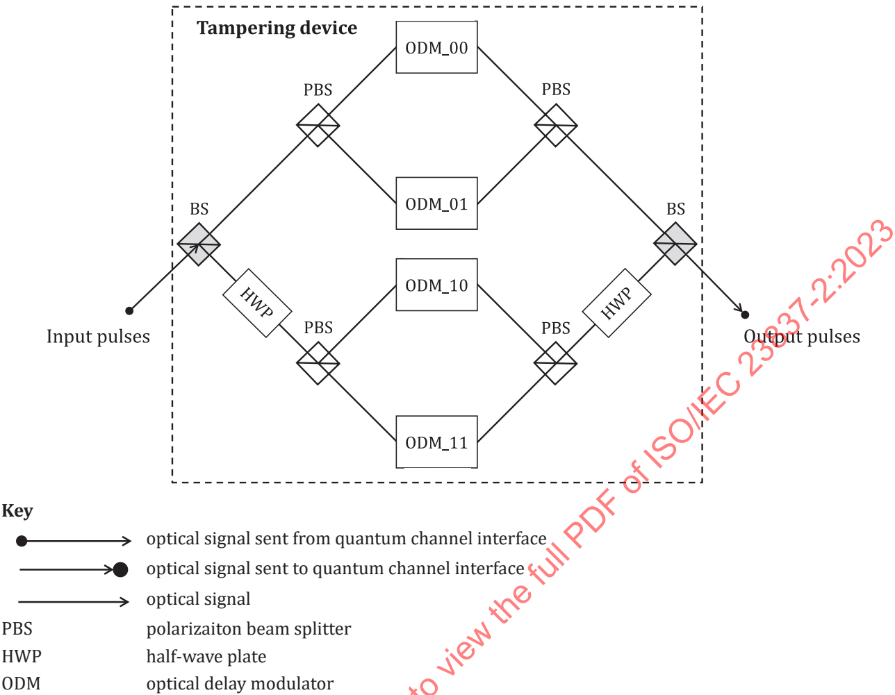
Figure 25 — Schematic of a setup for a possible instantiation of tampering device
