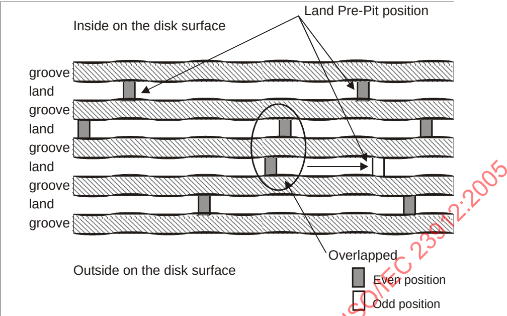
Figure 43 - Layout of land Pre-pit positioning
