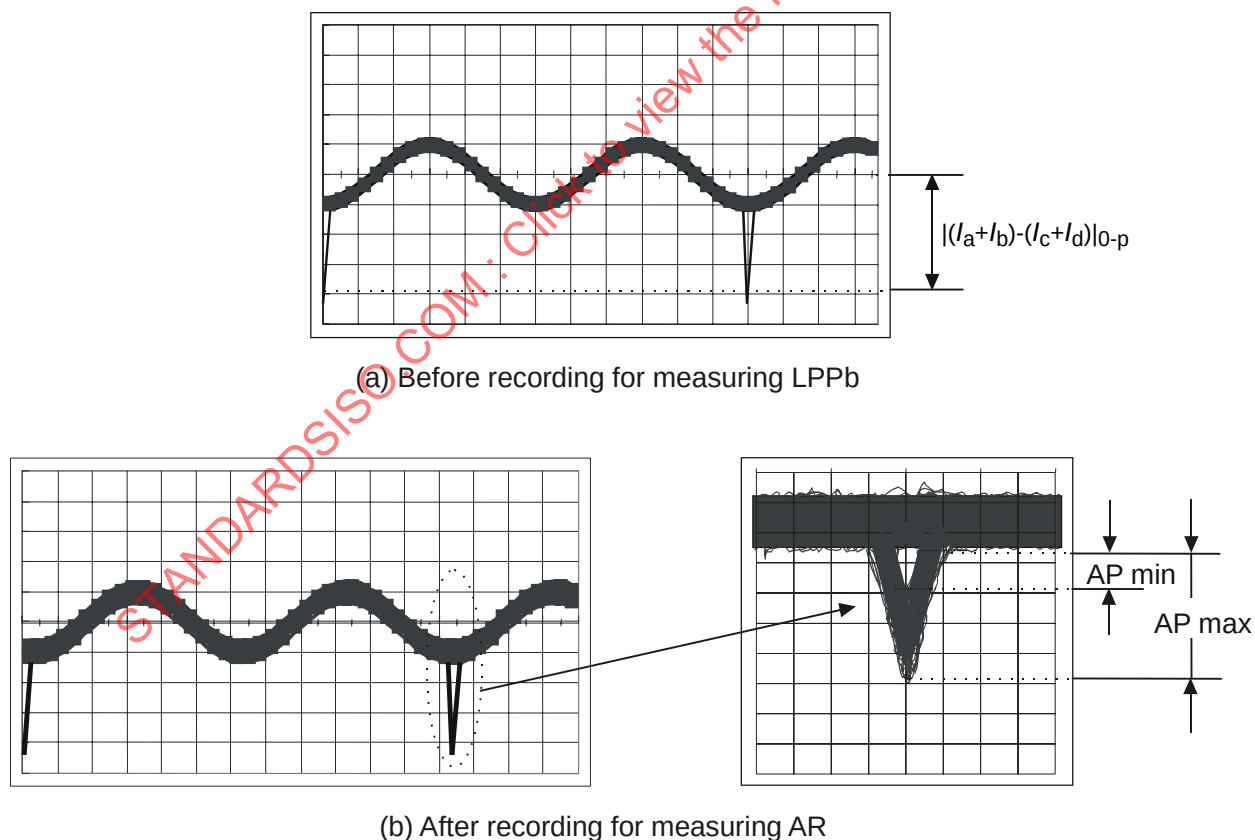
Figure 20 - Land Pre-Pit signal
