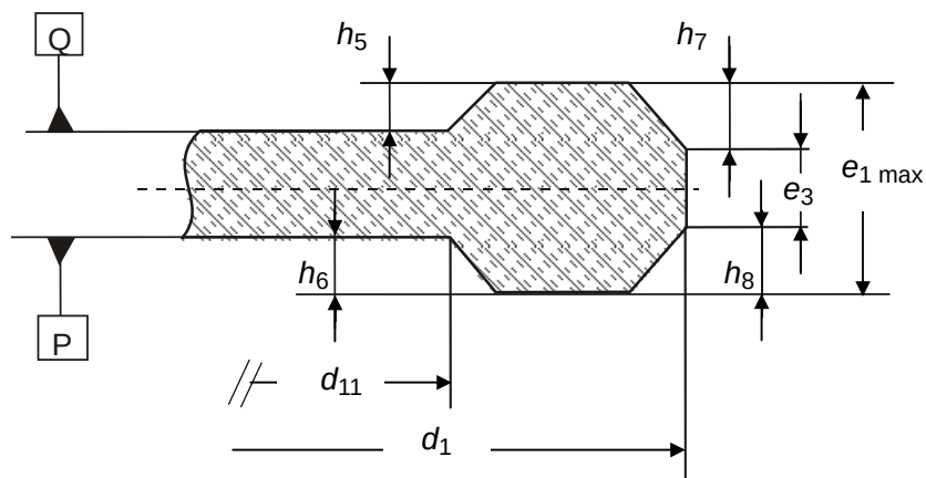
Figure 7 - Rim area
