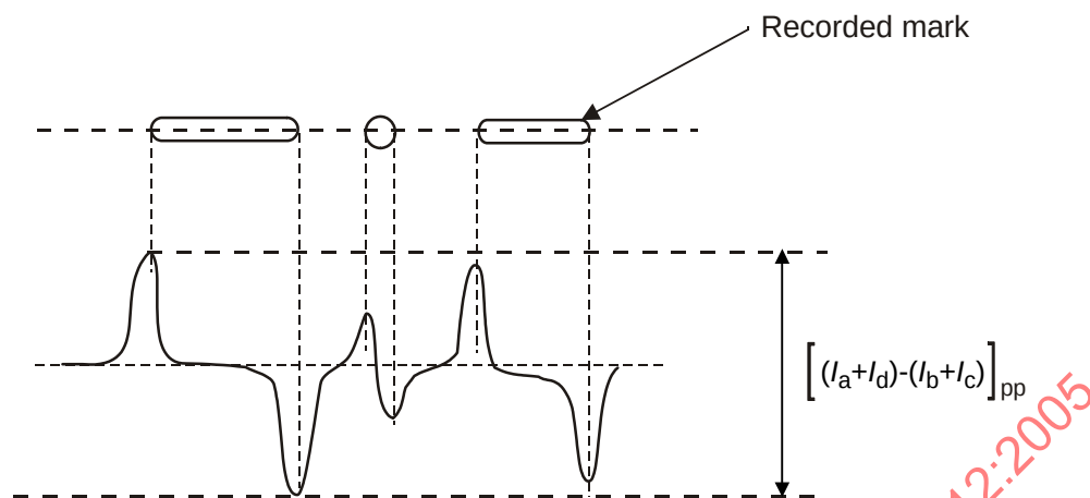
Figure 14 - Tangential push-pull signal
