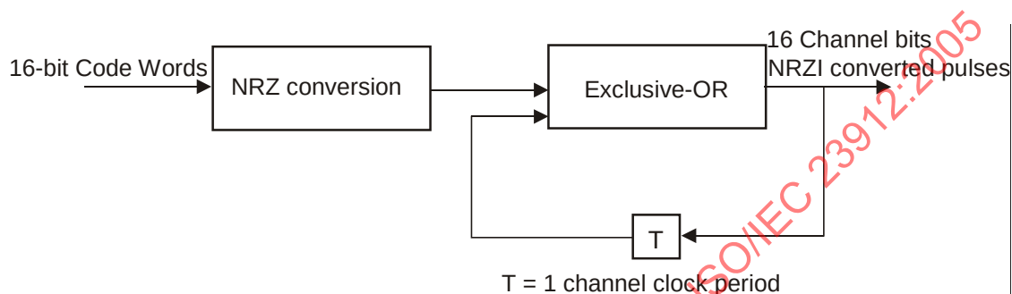
Figure 29 - NRZI conversion
