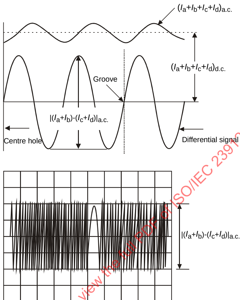
Figure 19. Radial push-pull tracking error signal
