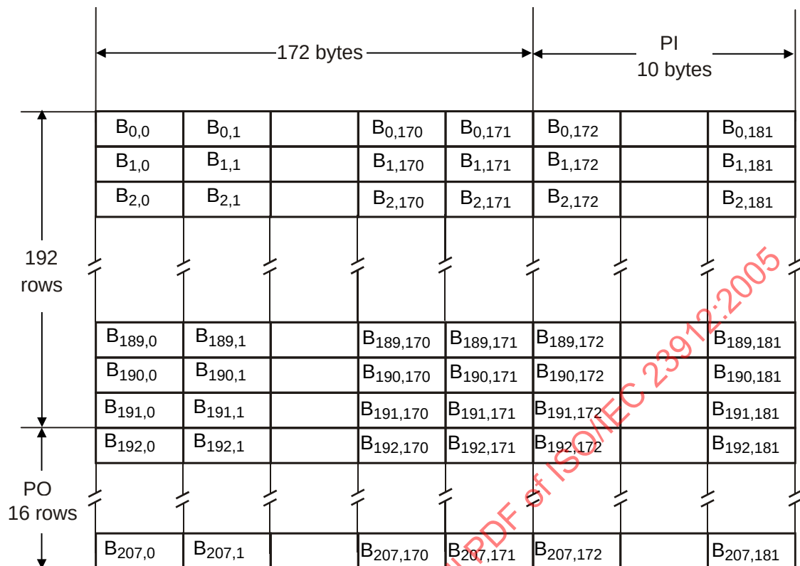
Figure 27 – ECC Block
