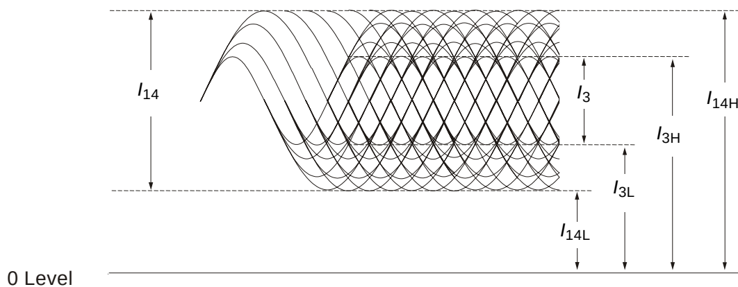
Figure 10 - Modulated amplitude
